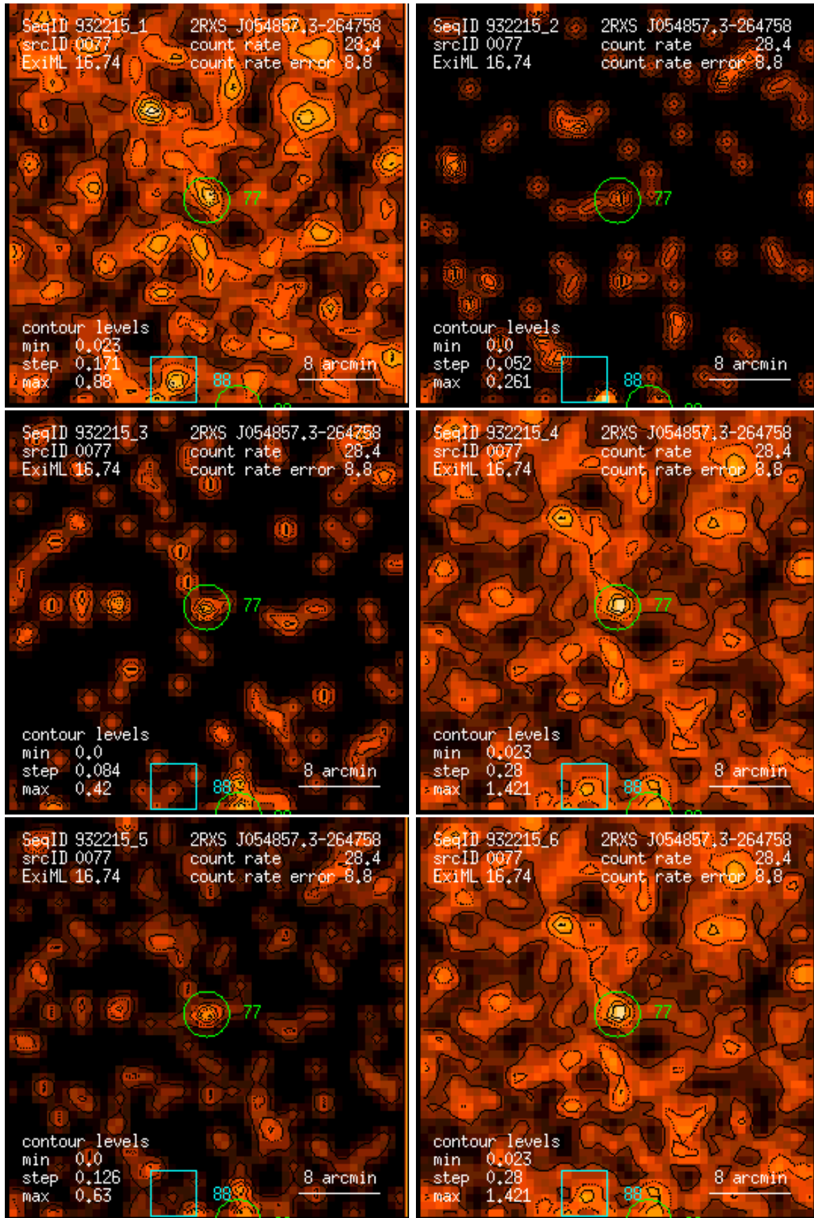
Figure 77: RASS 932215: detection 0077: band rate images, Gaussian filter: (1) PSPC channels 11 – 41, (2) 52 – 90, (3) 91 – 201, (4) 11 – 235, (5) 52 – 201, (6) 11 – 201. Broad band rates in counts/ks. Band rate contour levels in counts/ks/arcmin 2 .
