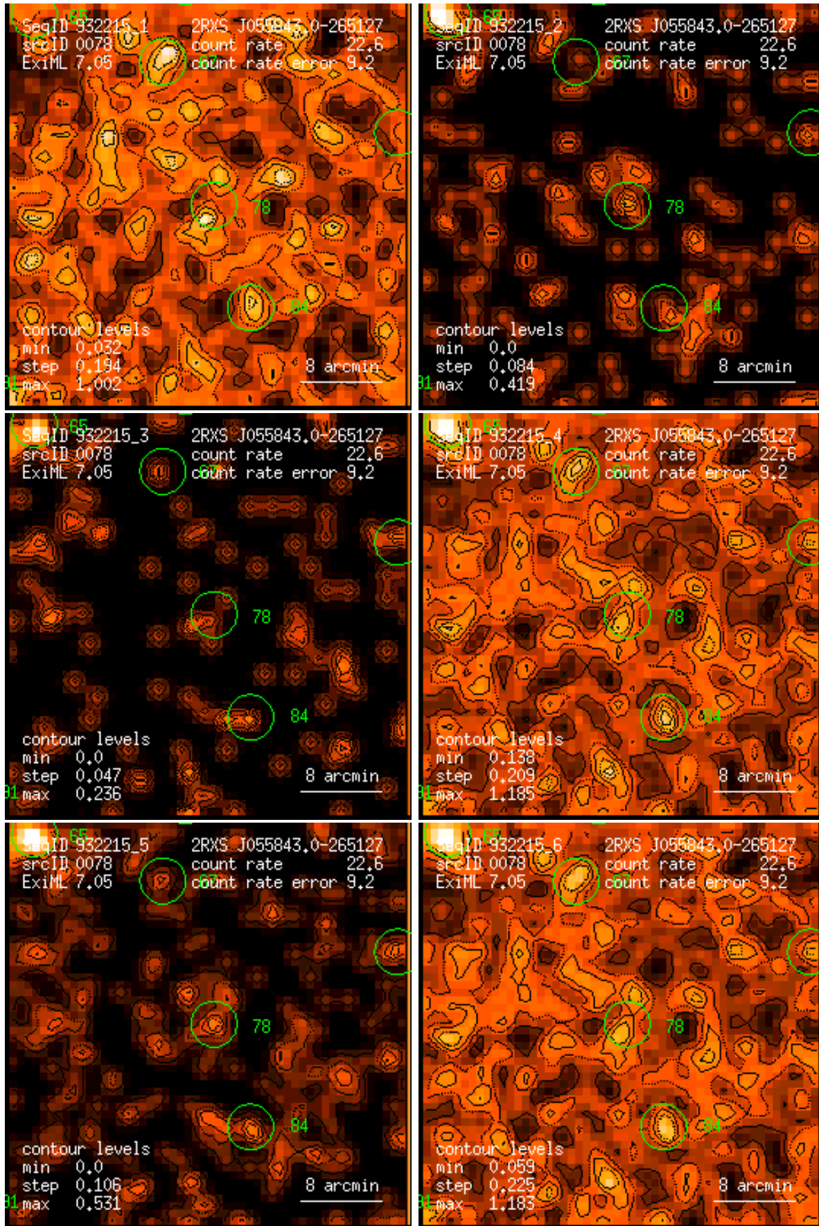
Figure 78: RASS 932215: detection 0078: band rate images, Gaussian filter: (1) PSPC channels 11 – 41, (2) 52 – 90, (3) 91 – 201, (4) 11 – 235, (5) 52 – 201, (6) 11 – 201. Broad band rates in counts/ks. Band rate contour levels in counts/ks/arcmin 2 .
