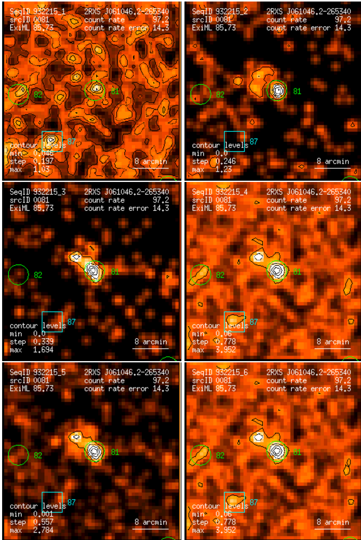
Figure 81: RASS 932215: detection 0081: band rate images, Gaussian filter: (1) PSPC channels 11 – 41, (2) 52 – 90, (3) 91 – 201, (4) 11 – 235, (5) 52 – 201, (6) 11 – 201. Broad band rates in counts/ks. Band rate contour levels in counts/ks/arcmin 2 .
