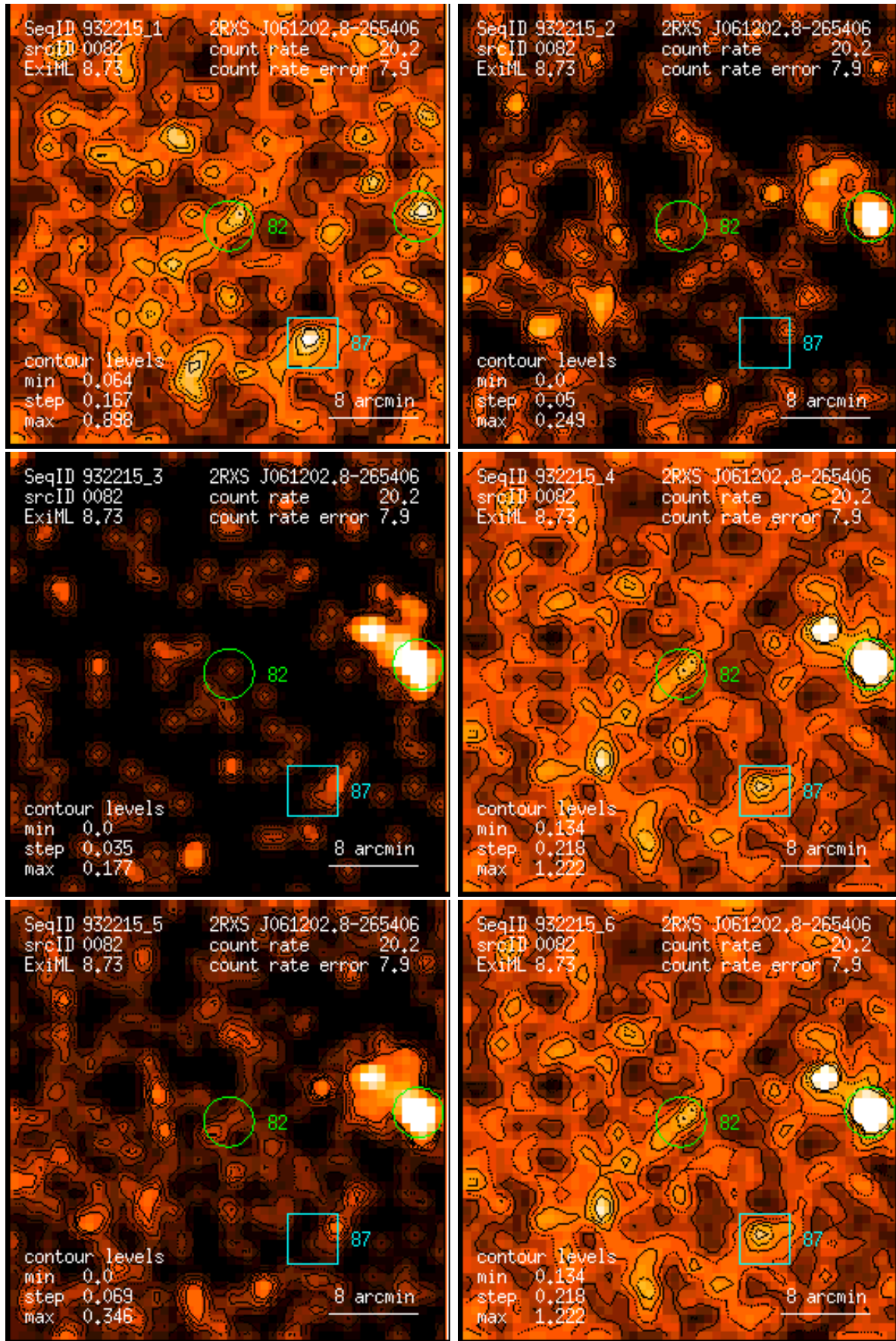
Figure 82: RASS 932215: detection 0082: band rate images, Gaussian filter: (1) PSPC channels 11 – 41, (2) 52 – 90, (3) 91 – 201, (4) 11 – 235, (5) 52 – 201, (6) 11 – 201. Broad band rates in counts/ks. Band rate contour levels in counts/ks/arcmin 2 .
