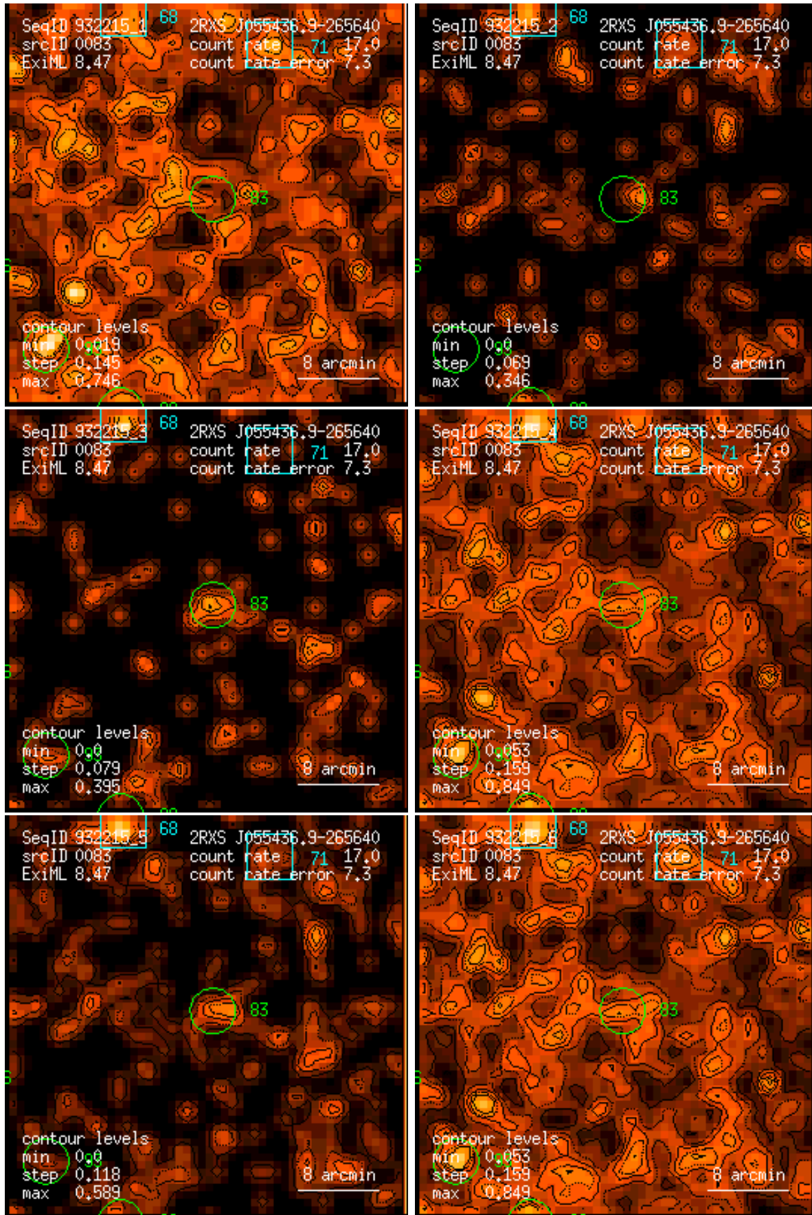
Figure 83: RASS 932215: detection 0083: band rate images, Gaussian filter: (1) PSPC channels 11 – 41, (2) 52 – 90, (3) 91 – 201, (4) 11 – 235, (5) 52 – 201, (6) 11 – 201. Broad band rates in counts/ks. Band rate contour levels in counts/ks/arcmin 2 .
