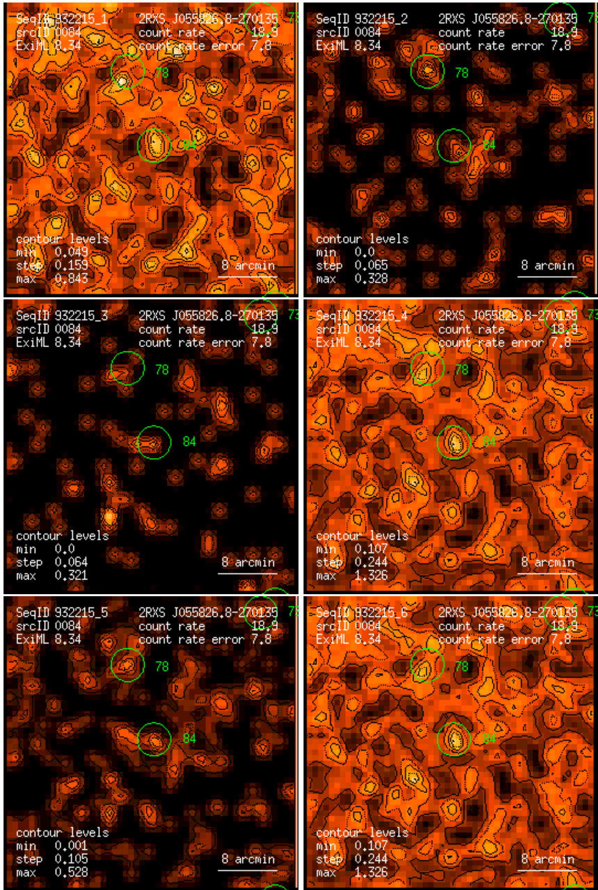
Figure 84: RASS 932215: detection 0084: band rate images, Gaussian filter: (1) PSPC channels 11 – 41, (2) 52 – 90, (3) 91 – 201, (4) 11 – 235, (5) 52 – 201, (6) 11 – 201. Broad band rates in counts/ks. Band rate contour levels in counts/ks/arcmin 2 .
