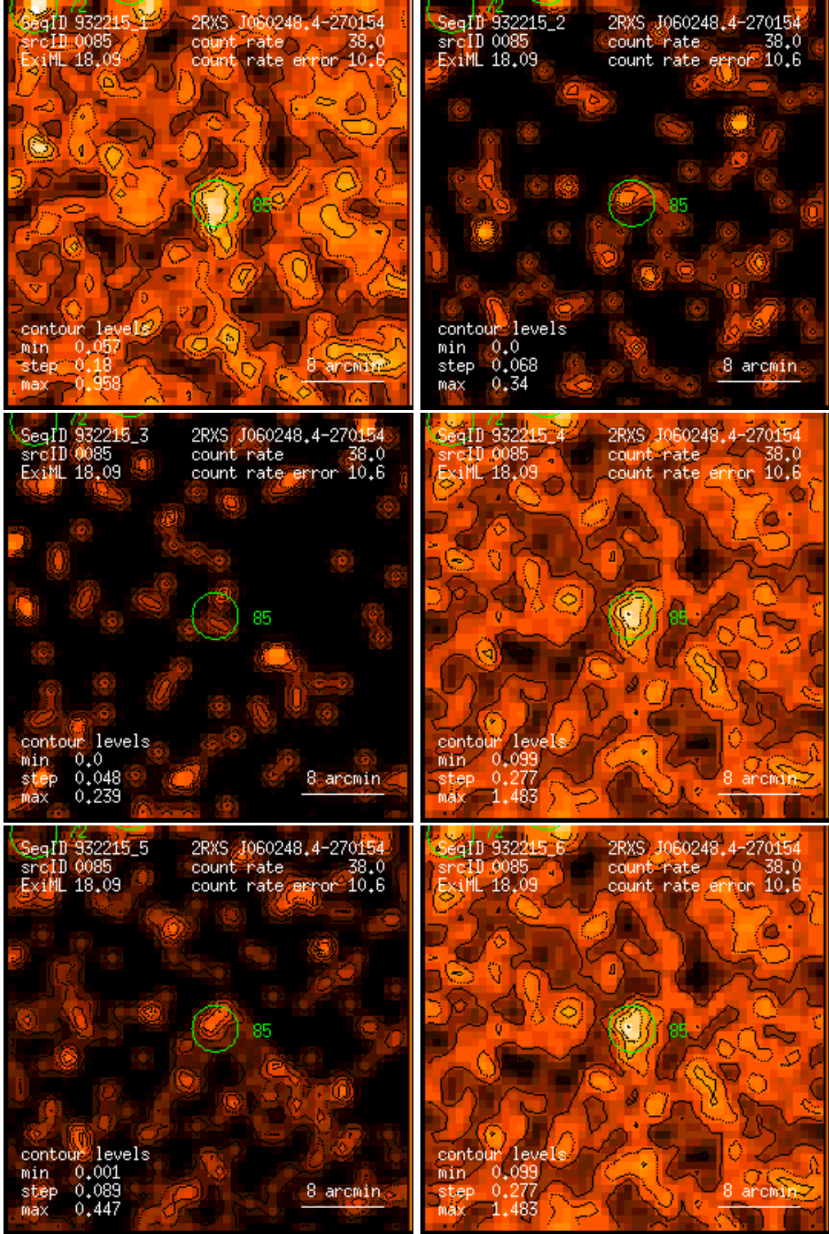
Figure 85: RASS 932215: detection 0085: band rate images, Gaussian filter: (1) PSPC channels 11 – 41, (2) 52 – 90, (3) 91 – 201, (4) 11 – 235, (5) 52 – 201, (6) 11 – 201. Broad band rates in counts/ks. Band rate contour levels in counts/ks/arcmin 2 .
