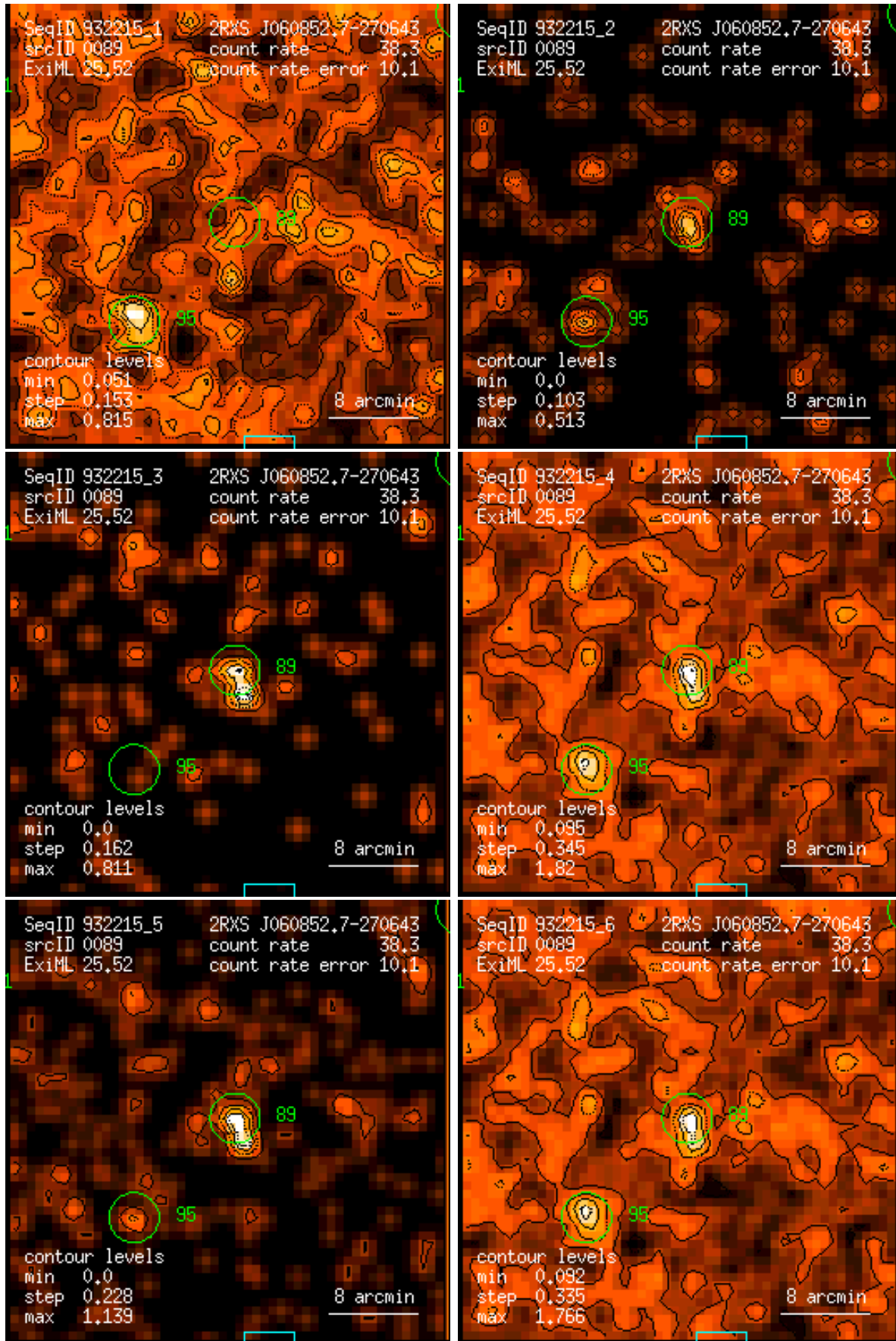
Figure 89: RASS 932215: detection 0089: band rate images, Gaussian filter: (1) PSPC channels 11 – 41, (2) 52 – 90, (3) 91 – 201, (4) 11 – 235, (5) 52 – 201, (6) 11 – 201. Broad band rates in counts/ks. Band rate contour levels in counts/ks/arcmin 2 .
