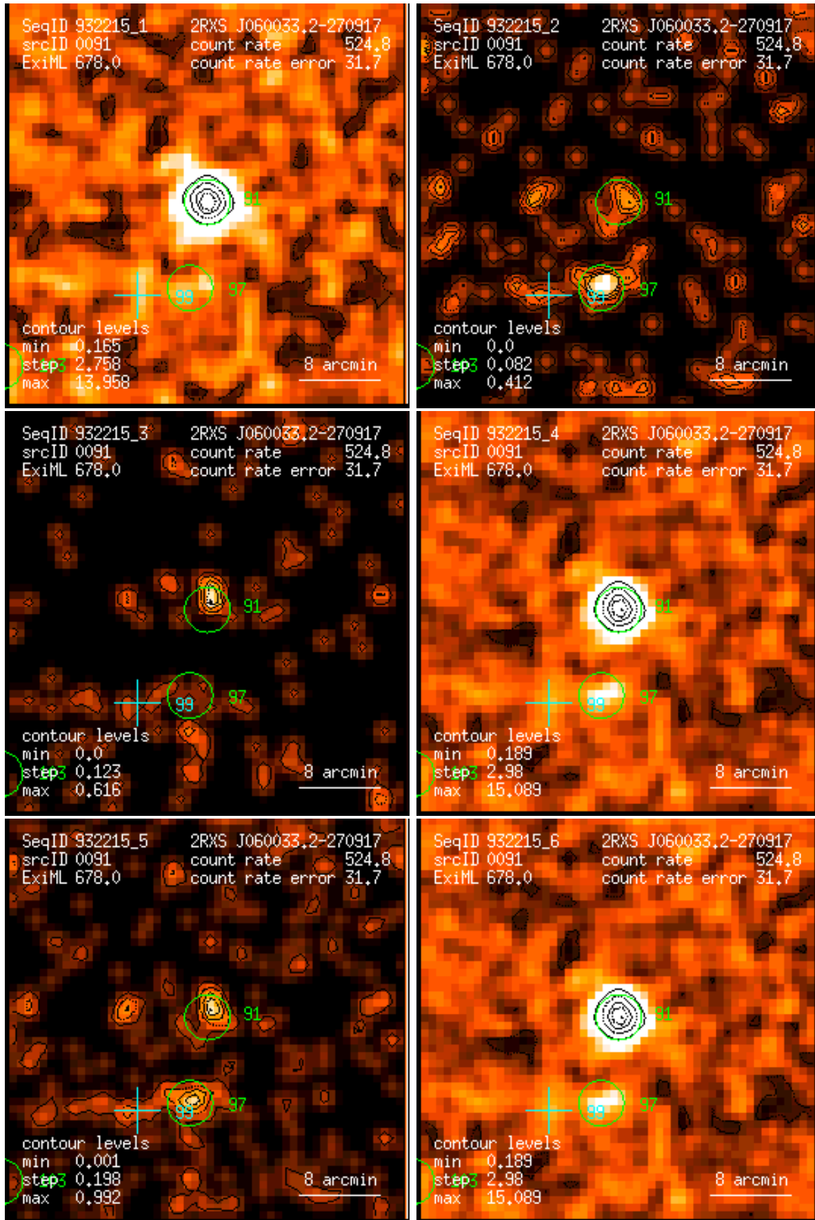
Figure 91: RASS 932215: detection 0091: band rate images, Gaussian filter: (1) PSPC channels 11 – 41, (2) 52 – 90, (3) 91 – 201, (4) 11 – 235, (5) 52 – 201, (6) 11 – 201. Broad band rates in counts/ks. Band rate contour levels in counts/ks/arcmin 2 .
