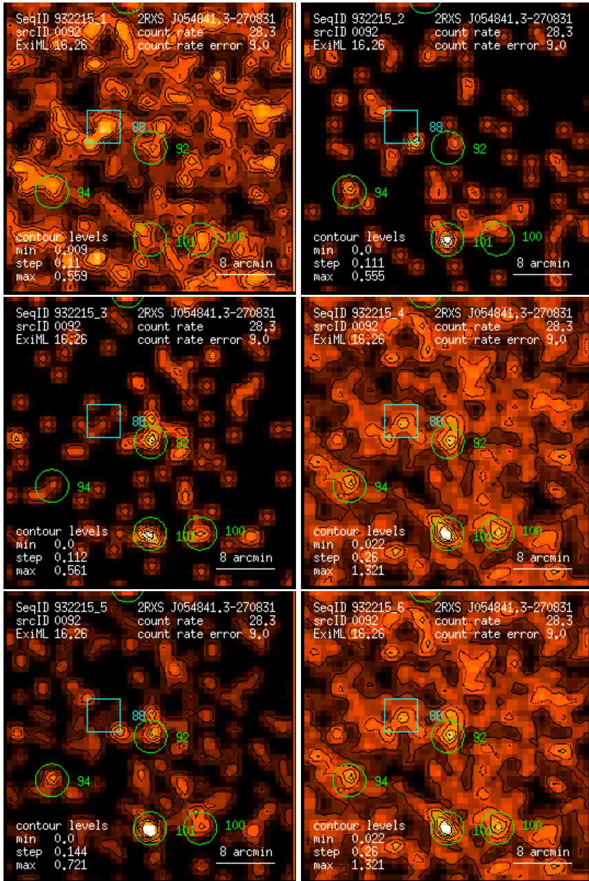
Figure 92: RASS 932215: detection 0092: band rate images, Gaussian filter: (1) PSPC channels 11 – 41, (2) 52 – 90, (3) 91 – 201, (4) 11 – 235, (5) 52 – 201, (6) 11 – 201. Broad band rates in counts/ks. Band rate contour levels in counts/ks/arcmin 2 .
