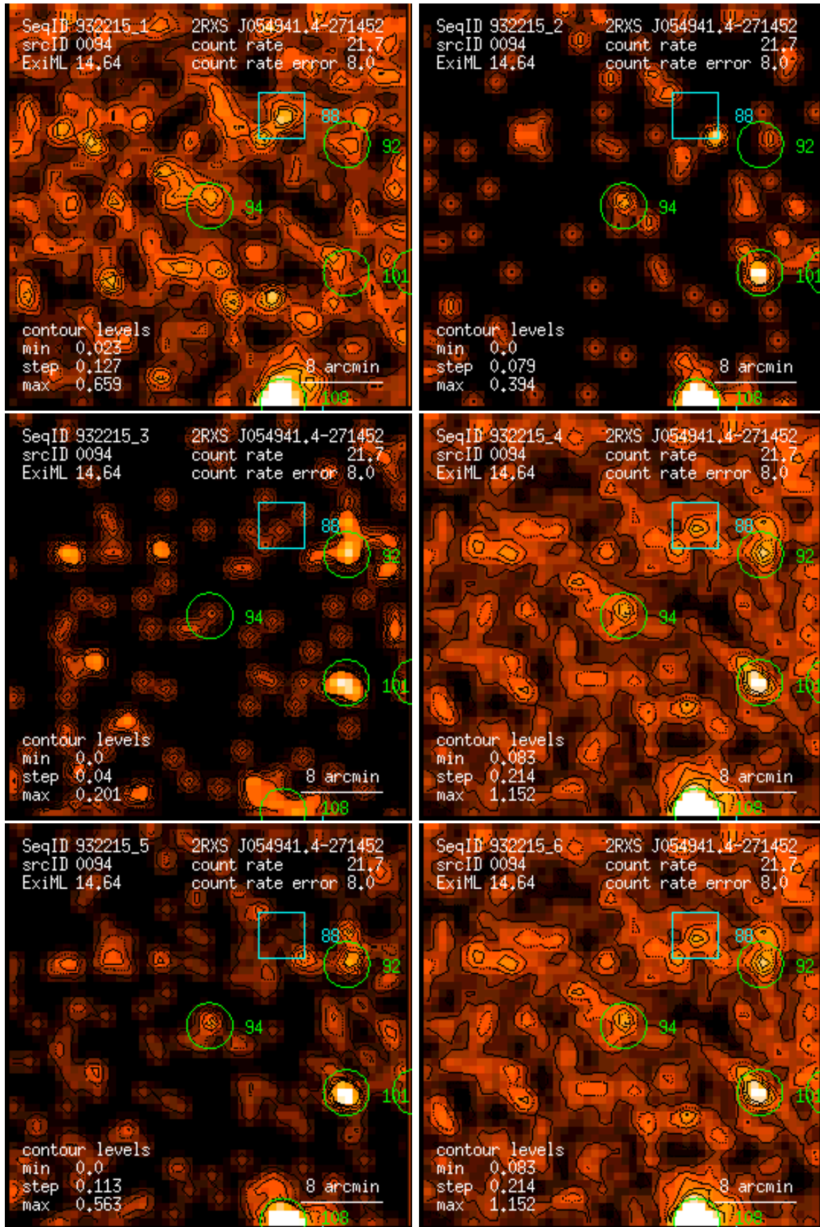
Figure 94: RASS 932215: detection 0094: band rate images, Gaussian filter: (1) PSPC channels 11 – 41, (2) 52 – 90, (3) 91 – 201, (4) 11 – 235, (5) 52 – 201, (6) 11 – 201. Broad band rates in counts/ks. Band rate contour levels in counts/ks/arcmin 2 .
