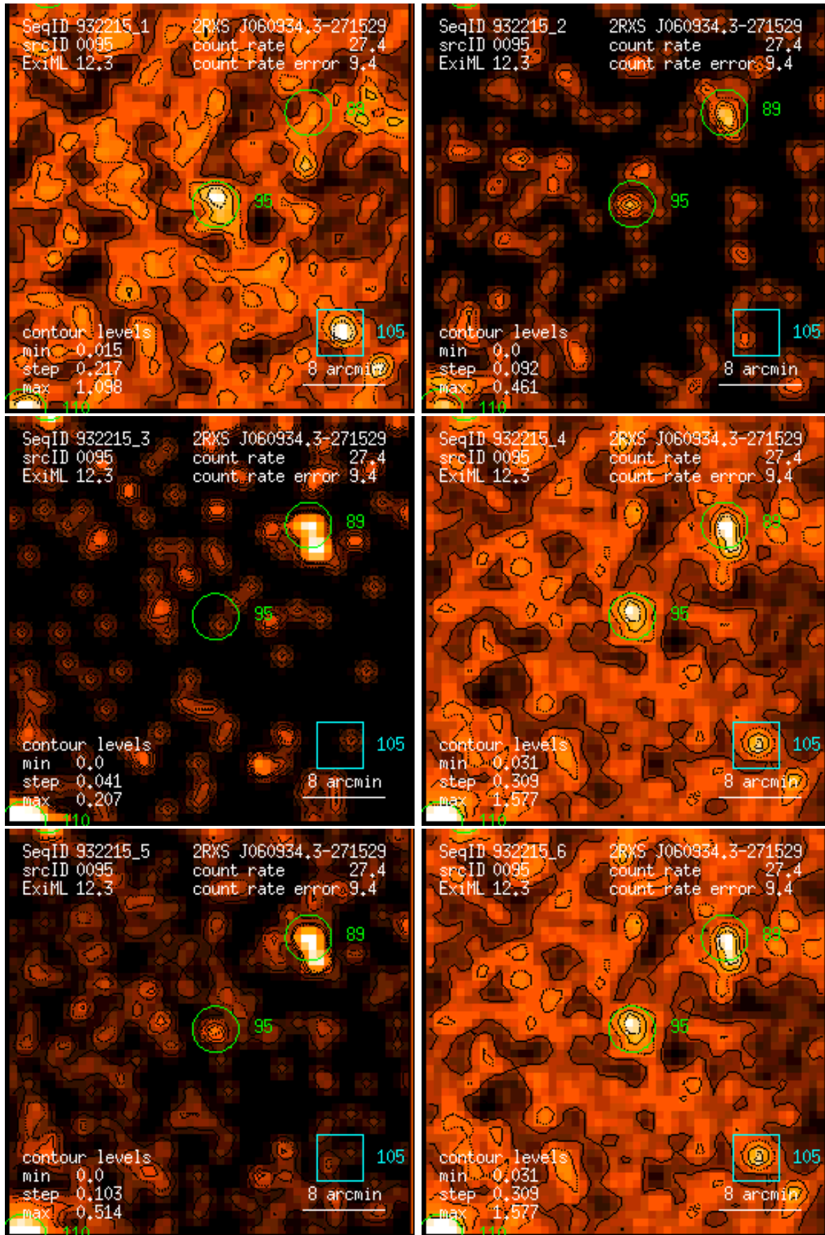
Figure 95: RASS 932215: detection 0095: band rate images, Gaussian filter: (1) PSPC channels 11 – 41, (2) 52 – 90, (3) 91 – 201, (4) 11 – 235, (5) 52 – 201, (6) 11 – 201. Broad band rates in counts/ks. Band rate contour levels in counts/ks/arcmin 2 .
