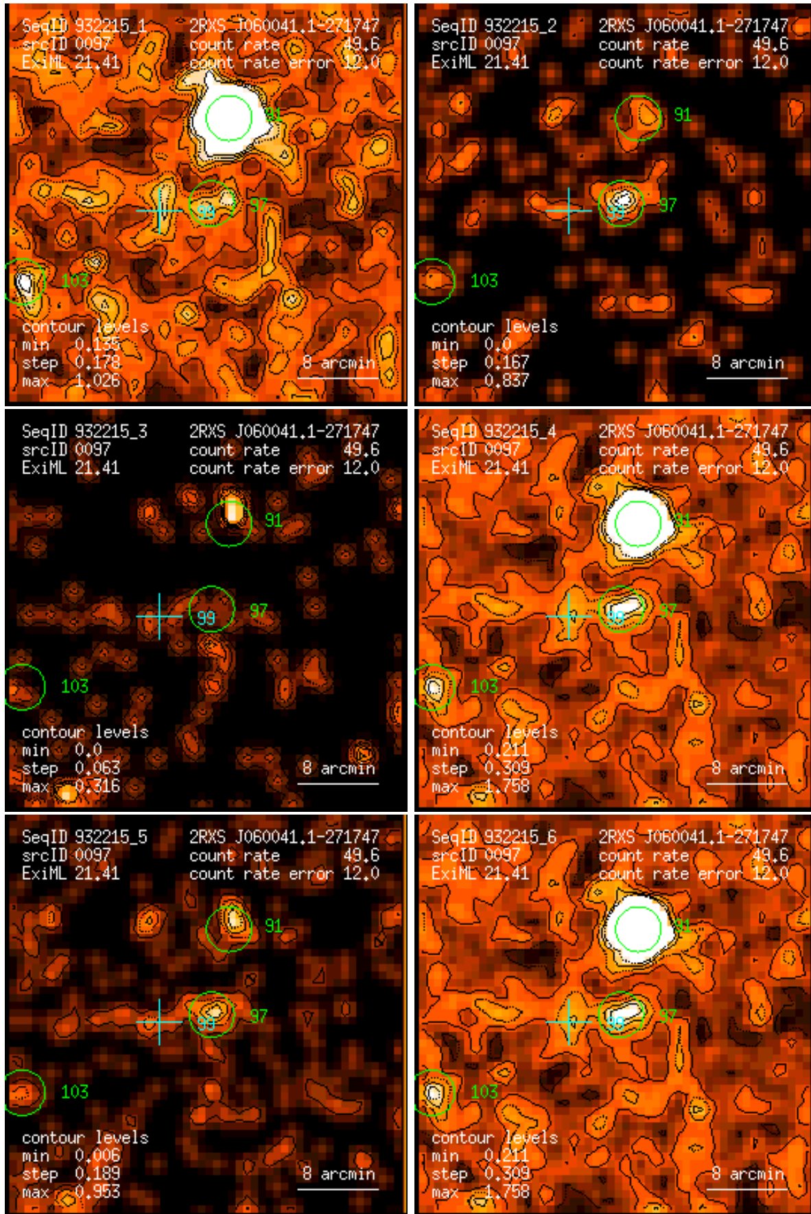
Figure 97: RASS 932215: detection 0097: band rate images, Gaussian filter: (1) PSPC channels 11 – 41, (2) 52 – 90, (3) 91 – 201, (4) 11 – 235, (5) 52 – 201, (6) 11 – 201. Broad band rates in counts/ks. Band rate contour levels in counts/ks/arcmin 2 .
