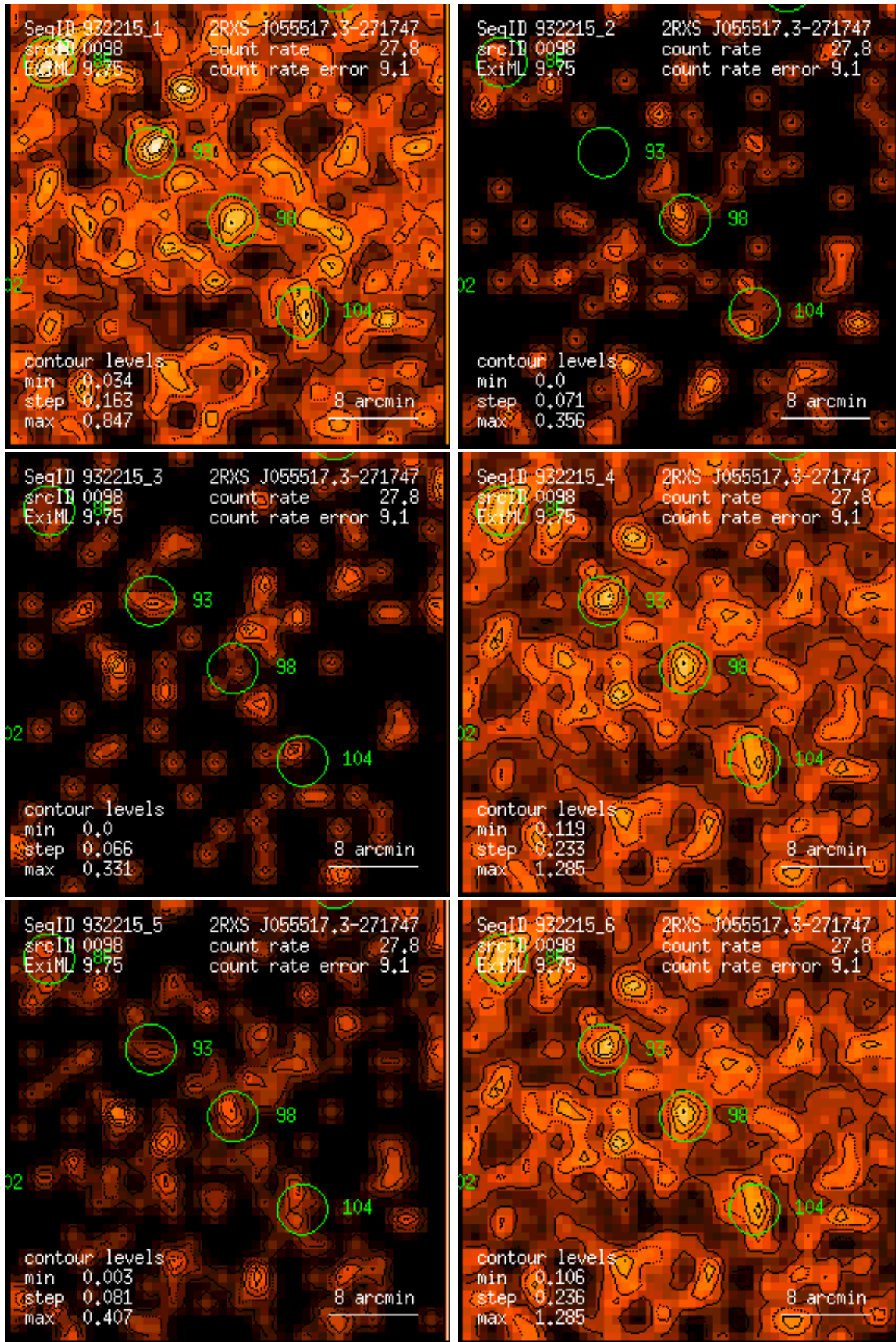
Figure 98: RASS 932215: detection 0098: band rate images, Gaussian filter: (1) PSPC channels 11 – 41, (2) 52 – 90, (3) 91 – 201, (4) 11 – 235, (5) 52 – 201, (6) 11 – 201. Broad band rates in counts/ks. Band rate contour levels in counts/ks/arcmin 2 .
