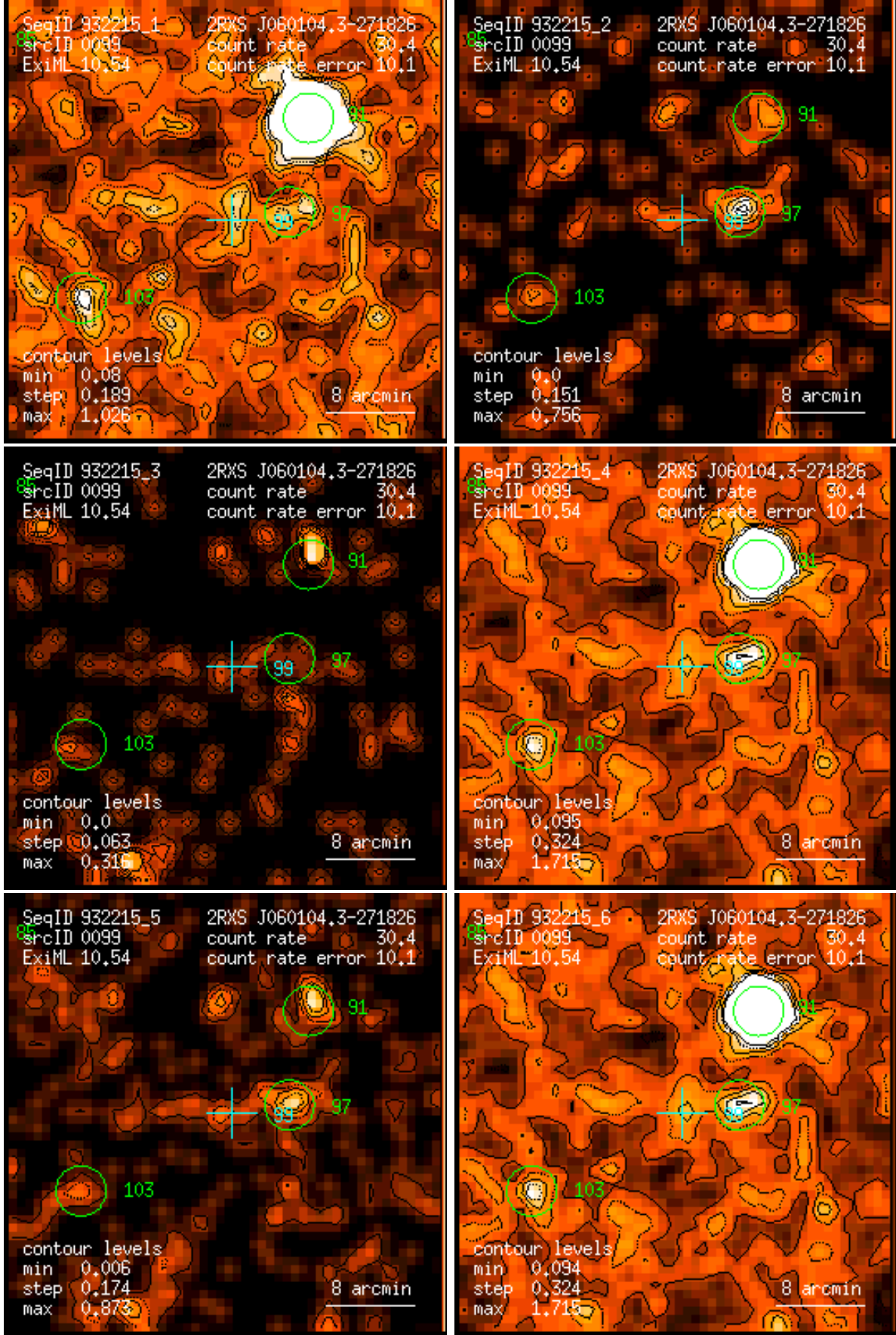
Figure 99: RASS 932215: detection 0099: band rate images, Gaussian filter: (1) PSPC channels 11 – 41, (2) 52 – 90, (3) 91 – 201, (4) 11 – 235, (5) 52 – 201, (6) 11 – 201. Broad band rates in counts/ks. Band rate contour levels in counts/ks/arcmin 2 .
