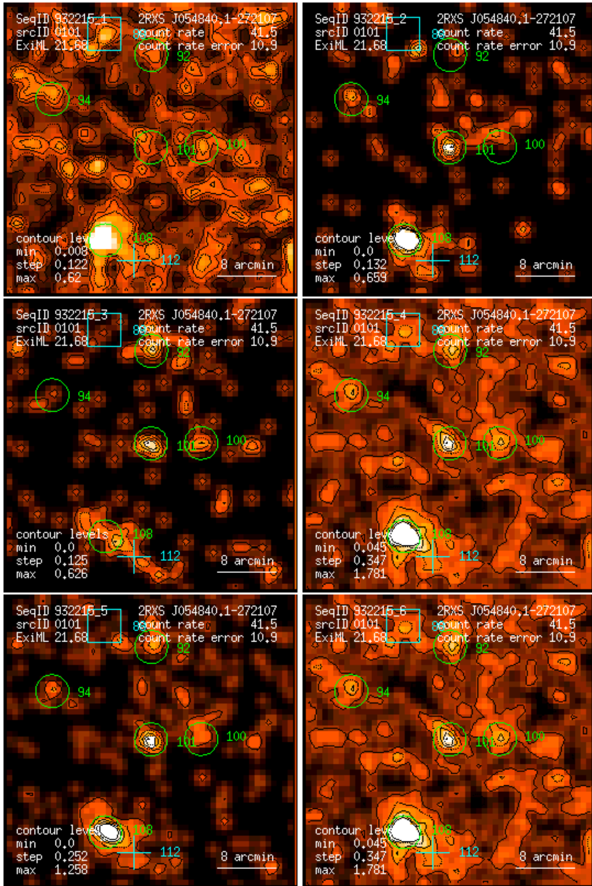
Figure 101: RASS 932215: detection 0101: band rate images, Gaussian filter: (1) PSPC channels 11 – 41, (2) 52 – 90, (3) 91 – 201, (4) 11 – 235, (5) 52 – 201, (6) 11 – 201. Broad band rates in counts/ks. Band rate contour levels in counts/ks/arcmin 2 .
