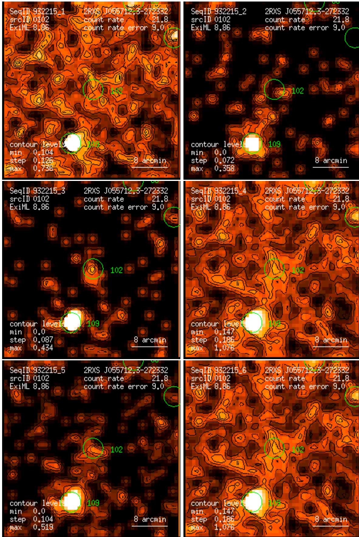
Figure 102: RASS 932215: detection 0102: band rate images, Gaussian filter: (1) PSPC channels 11 – 41, (2) 52 – 90, (3) 91 – 201, (4) 11 – 235, (5) 52 – 201, (6) 11 – 201. Broad band rates in counts/ks. Band rate contour levels in counts/ks/arcmin 2 .
