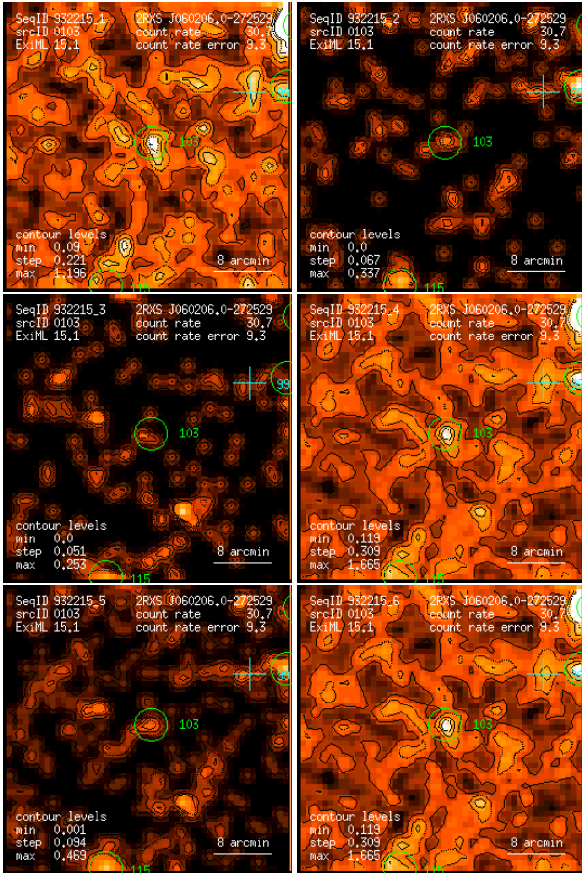
Figure 103: RASS 932215: detection 0103: band rate images, Gaussian filter: (1) PSPC channels 11 – 41, (2) 52 – 90, (3) 91 – 201, (4) 11 – 235, (5) 52 – 201, (6) 11 – 201. Broad band rates in counts/ks. Band rate contour levels in counts/ks/arcmin 2 .
