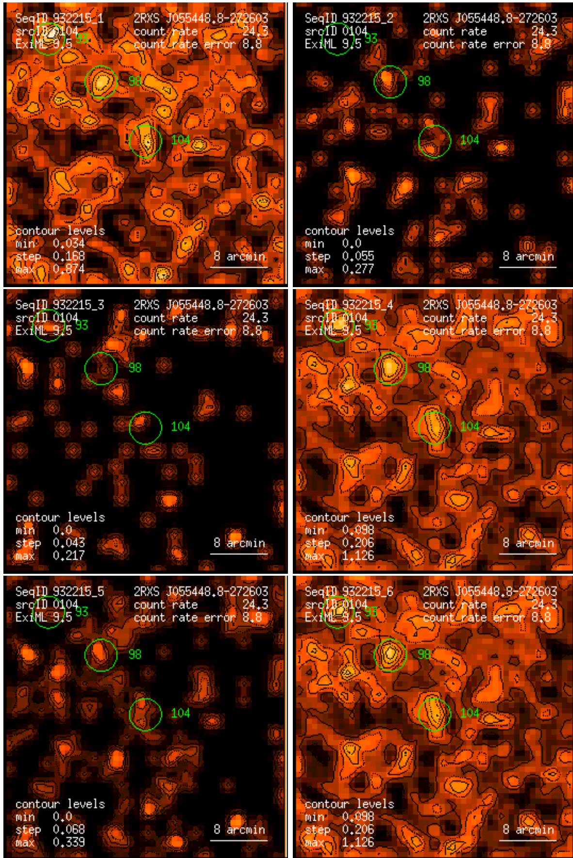
Figure 104: RASS 932215: detection 0104: band rate images, Gaussian filter: (1) PSPC channels 11 – 41, (2) 52 – 90, (3) 91 – 201, (4) 11 – 235, (5) 52 – 201, (6) 11 – 201. Broad band rates in counts/ks. Band rate contour levels in counts/ks/arcmin 2 .
