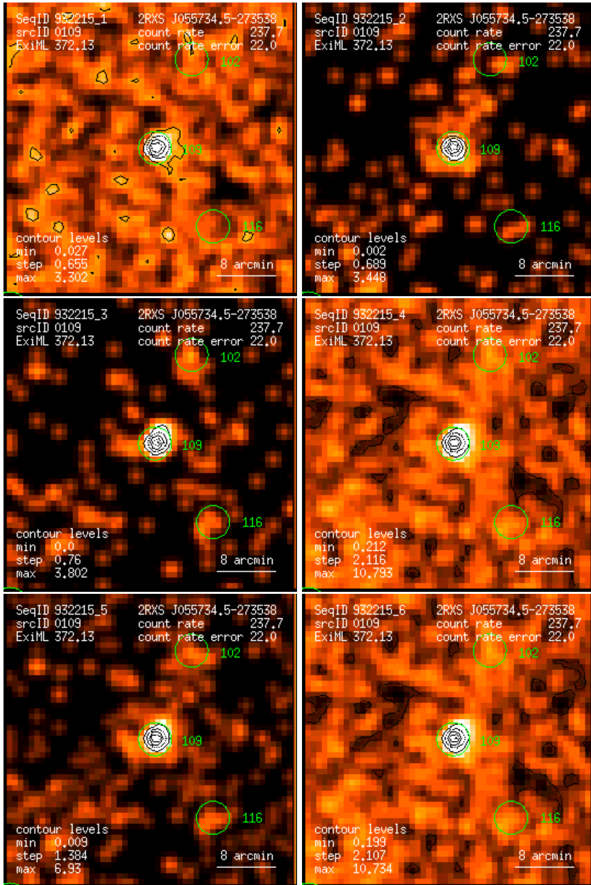
Figure 109: RASS 932215: detection 0109: band rate images, Gaussian filter: (1) PSPC channels 11 – 41, (2) 52 – 90, (3) 91 – 201, (4) 11 – 235, (5) 52 – 201, (6) 11 – 201. Broad band rates in counts/ks. Band rate contour levels in counts/ks/arcmin 2 .
