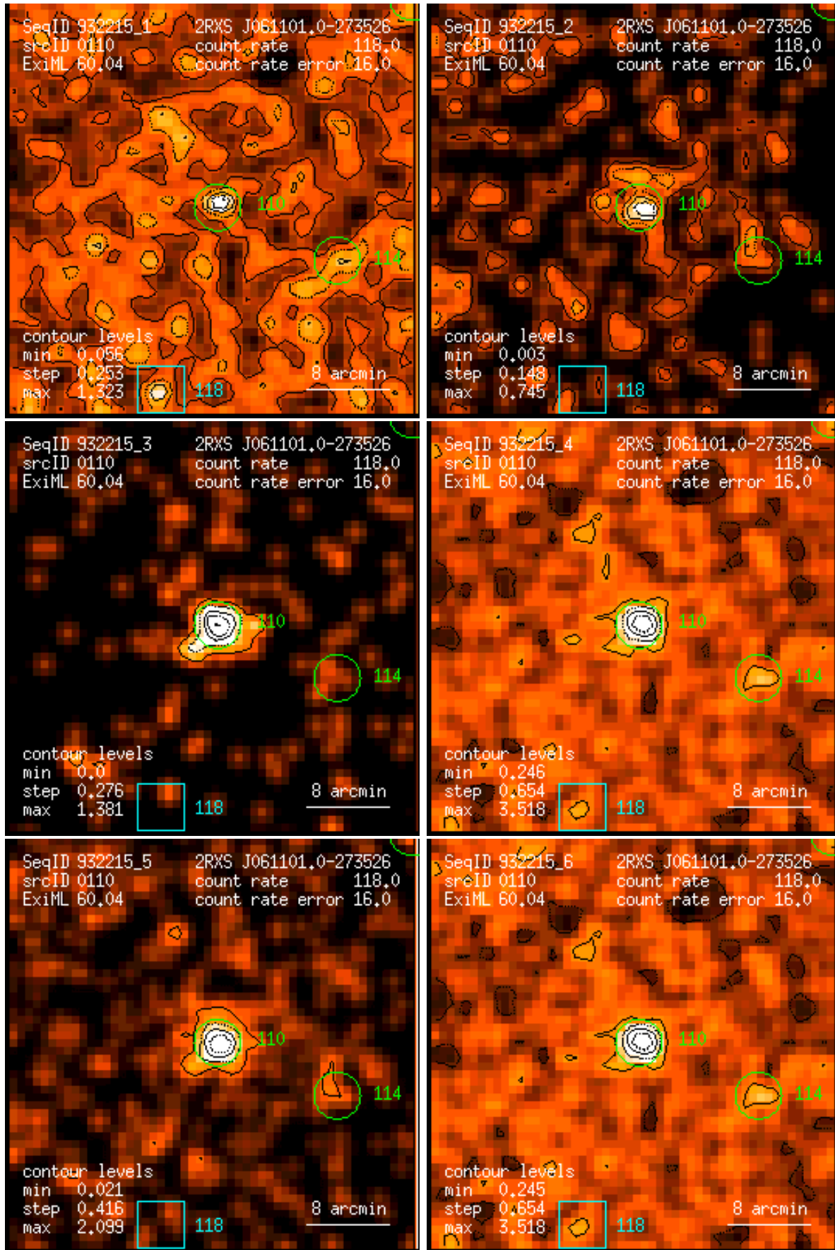
Figure 110: RASS 932215: detection 0110: band rate images, Gaussian filter: (1) PSPC channels 11 – 41, (2) 52 – 90, (3) 91 – 201, (4) 11 – 235, (5) 52 – 201, (6) 11 – 201. Broad band rates in counts/ks. Band rate contour levels in counts/ks/arcmin 2 .
