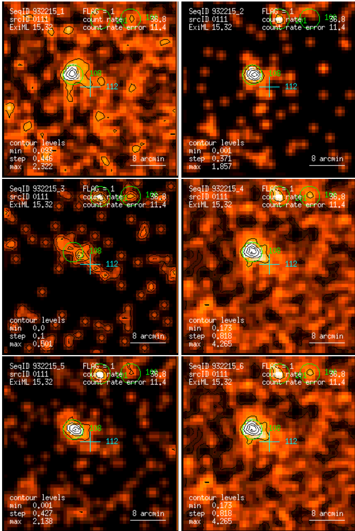
Figure 111: RASS 932215: detection 0111: band rate images, Gaussian filter: (1) PSPC channels 11 – 41, (2) 52 – 90, (3) 91 – 201, (4) 11 – 235, (5) 52 – 201, (6) 11 – 201. Broad band rates in counts/ks. Band rate contour levels in counts/ks/arcmin 2 .
