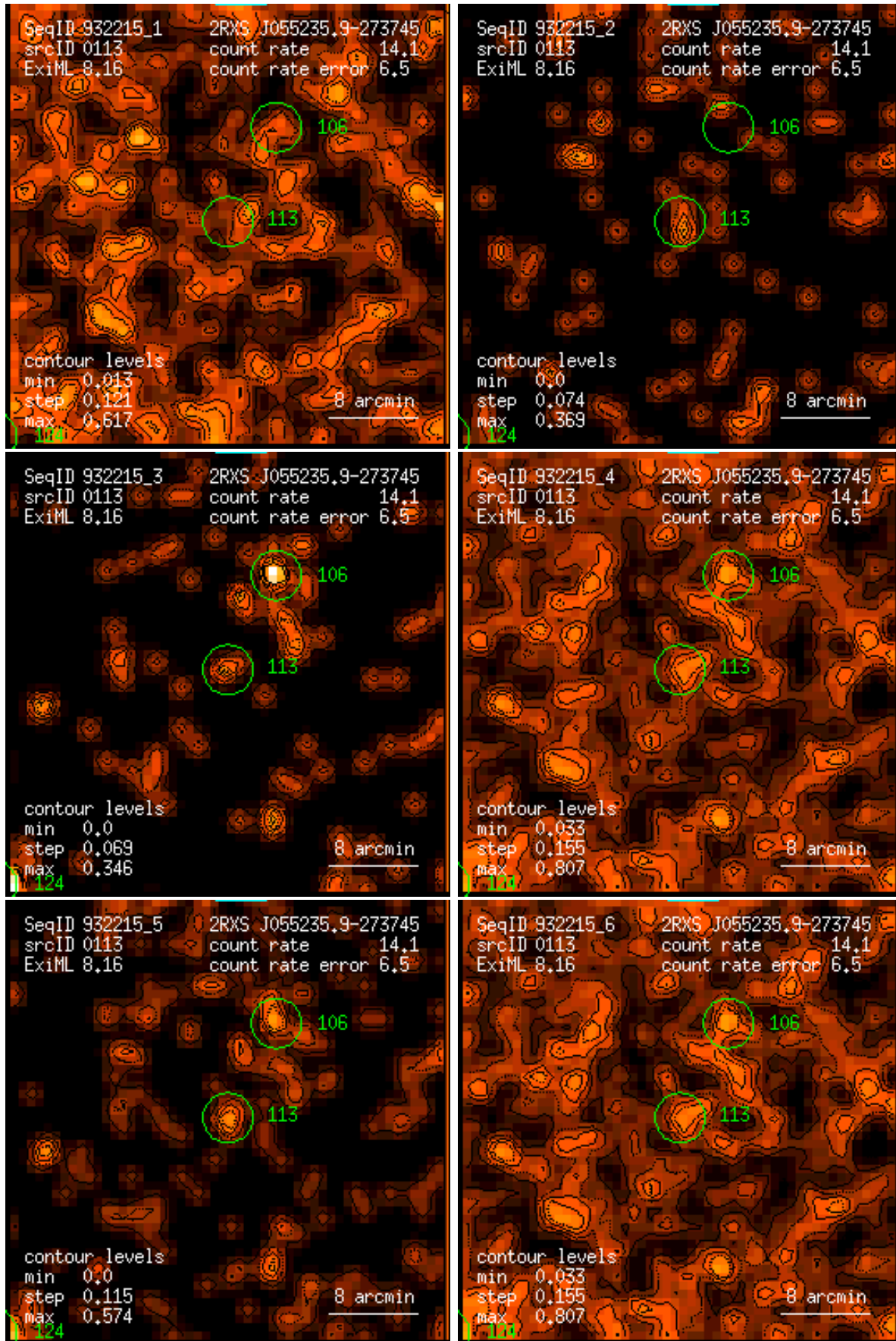
Figure 113: RASS 932215: detection 0113: band rate images, Gaussian filter: (1) PSPC channels 11 – 41, (2) 52 – 90, (3) 91 – 201, (4) 11 – 235, (5) 52 – 201, (6) 11 – 201. Broad band rates in counts/ks. Band rate contour levels in counts/ks/arcmin 2 .
