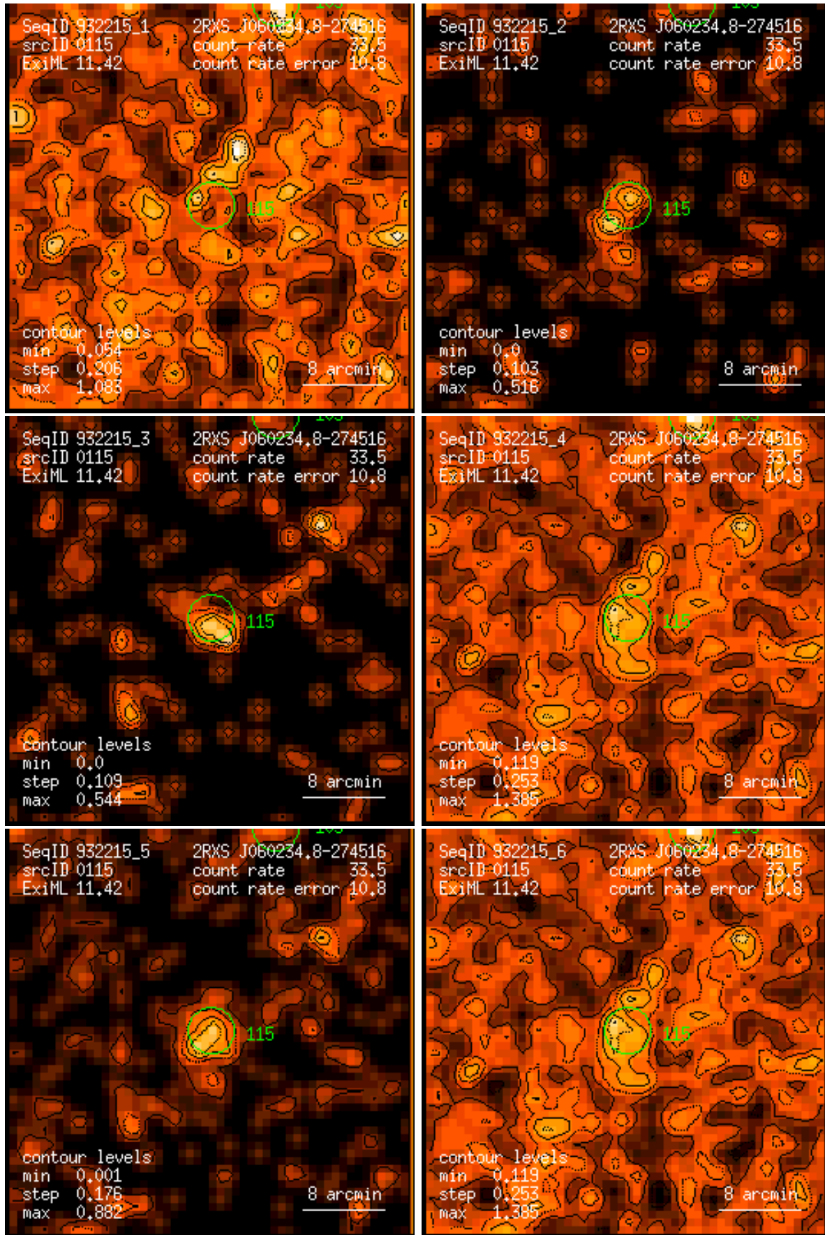
Figure 115: RASS 932215: detection 0115: band rate images, Gaussian filter: (1) PSPC channels 11 – 41, (2) 52 – 90, (3) 91 – 201, (4) 11 – 235, (5) 52 – 201, (6) 11 – 201. Broad band rates in counts/ks. Band rate contour levels in counts/ks/arcmin 2 .
