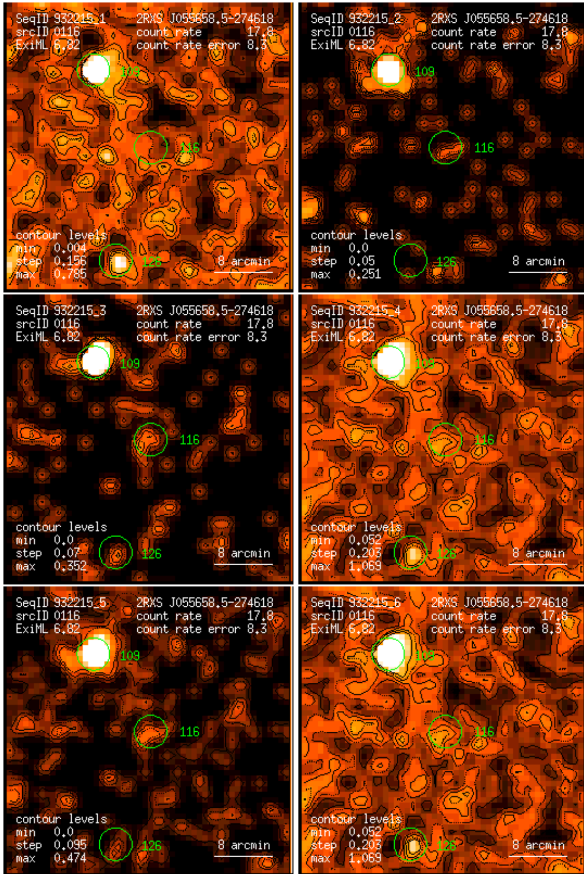
Figure 116: RASS 932215: detection 0116: band rate images, Gaussian filter: (1) PSPC channels 11 – 41, (2) 52 – 90, (3) 91 – 201, (4) 11 – 235, (5) 52 – 201, (6) 11 – 201. Broad band rates in counts/ks. Band rate contour levels in counts/ks/arcmin 2 .
