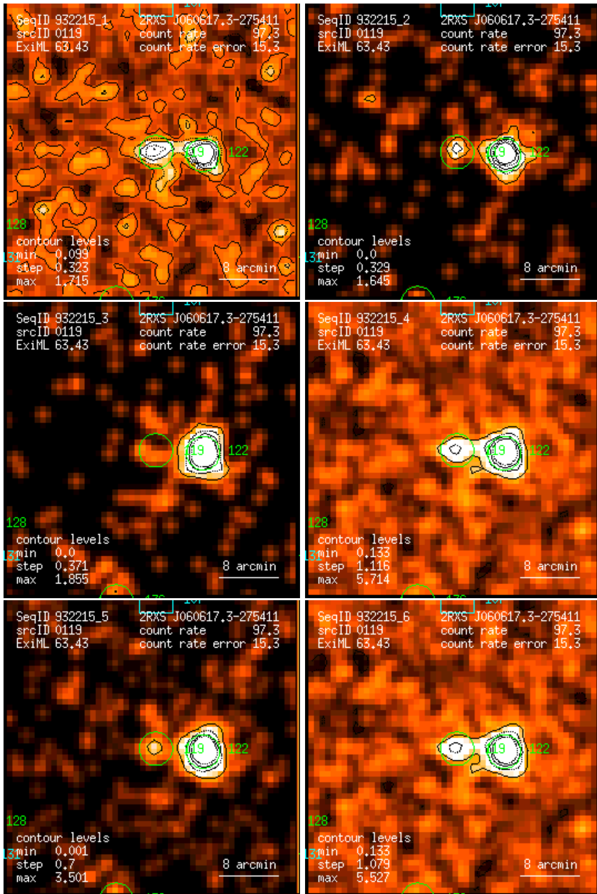
Figure 119: RASS 932215: detection 0119: band rate images, Gaussian filter: (1) PSPC channels 11 – 41, (2) 52 – 90, (3) 91 – 201, (4) 11 – 235, (5) 52 – 201, (6) 11 – 201. Broad band rates in counts/ks. Band rate contour levels in counts/ks/arcmin 2 .
