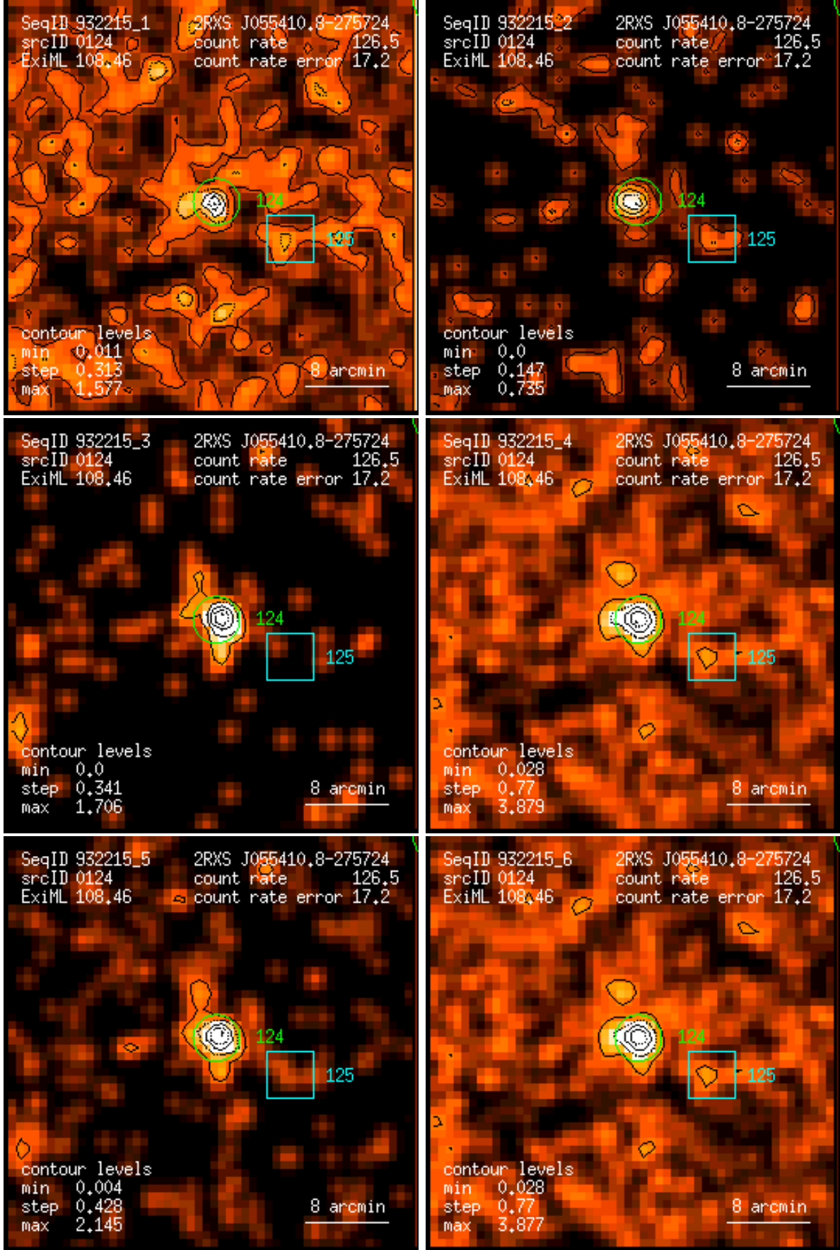
Figure 124: RASS 932215: detection 0124: band rate images, Gaussian filter: (1) PSPC channels 11 – 41, (2) 52 – 90, (3) 91 – 201, (4) 11 – 235, (5) 52 – 201, (6) 11 – 201. Broad band rates in counts/ks. Band rate contour levels in counts/ks/arcmin 2 .
