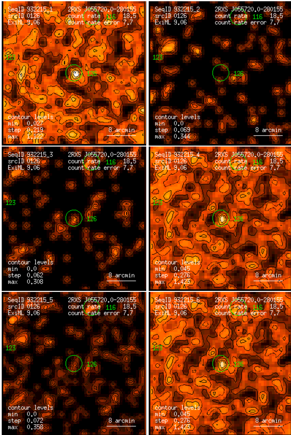
Figure 126: RASS 932215: detection 0126: band rate images, Gaussian filter: (1) PSPC channels 11 – 41, (2) 52 – 90, (3) 91 – 201, (4) 11 – 235, (5) 52 – 201, (6) 11 – 201. Broad band rates in counts/ks. Band rate contour levels in counts/ks/arcmin 2 .
