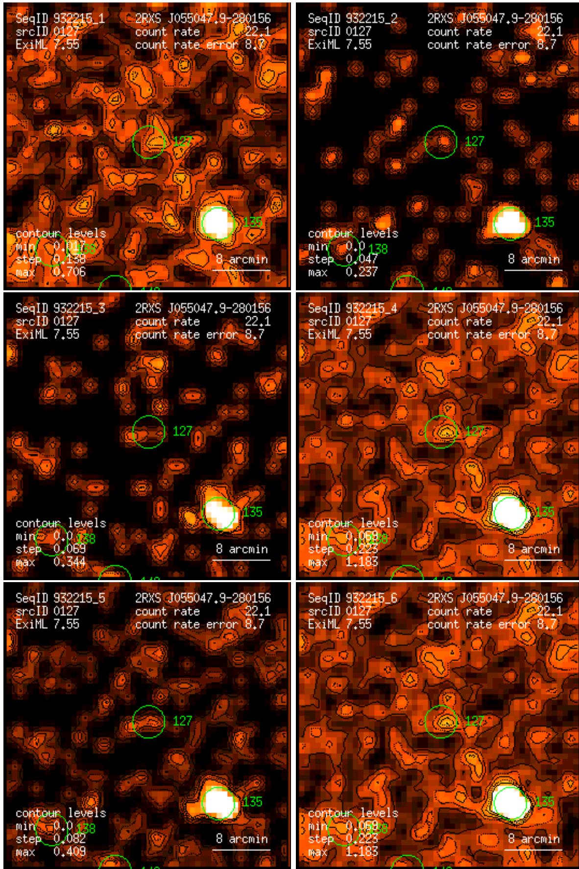
Figure 127: RASS 932215: detection 0127: band rate images, Gaussian filter: (1) PSPC channels 11 – 41, (2) 52 – 90, (3) 91 – 201, (4) 11 – 235, (5) 52 – 201, (6) 11 – 201. Broad band rates in counts/ks. Band rate contour levels in counts/ks/arcmin 2 .
