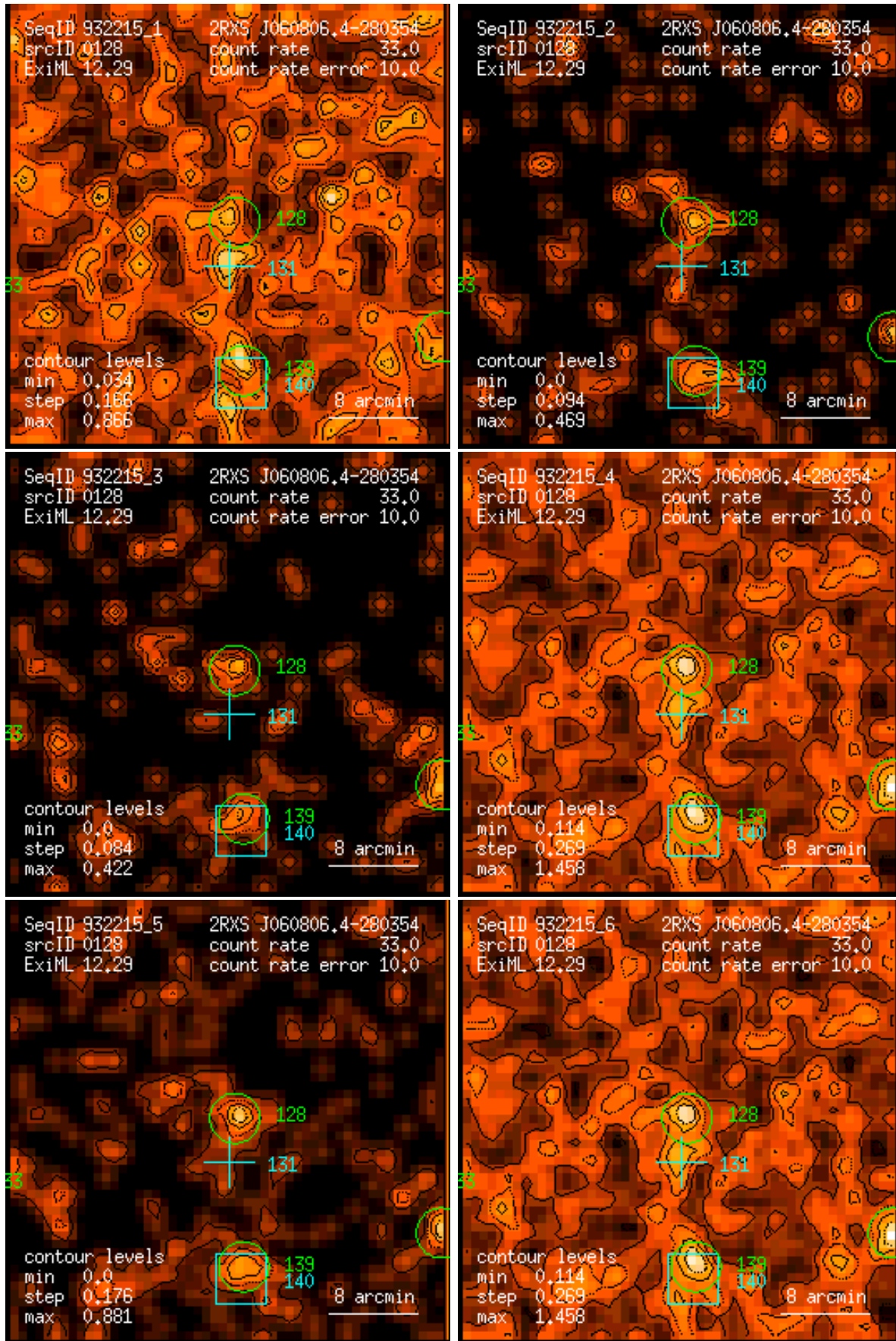
Figure 128: RASS 932215: detection 0128: band rate images, Gaussian filter: (1) PSPC channels 11 – 41, (2) 52 – 90, (3) 91 – 201, (4) 11 – 235, (5) 52 – 201, (6) 11 – 201. Broad band rates in counts/ks. Band rate contour levels in counts/ks/arcmin 2 .
