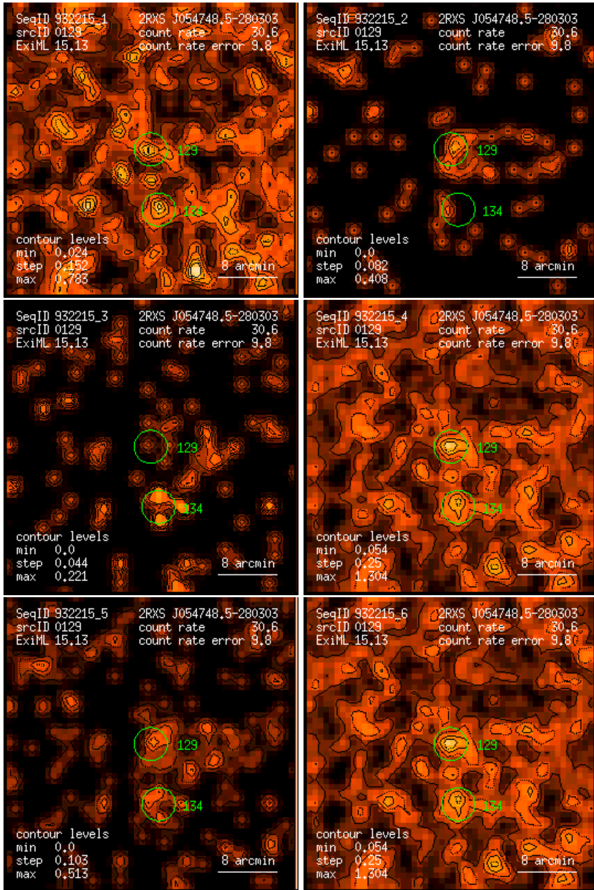
Figure 129: RASS 932215: detection 0129: band rate images, Gaussian filter: (1) PSPC channels 11 – 41, (2) 52 – 90, (3) 91 – 201, (4) 11 – 235, (5) 52 – 201, (6) 11 – 201. Broad band rates in counts/ks. Band rate contour levels in counts/ks/arcmin 2 .
