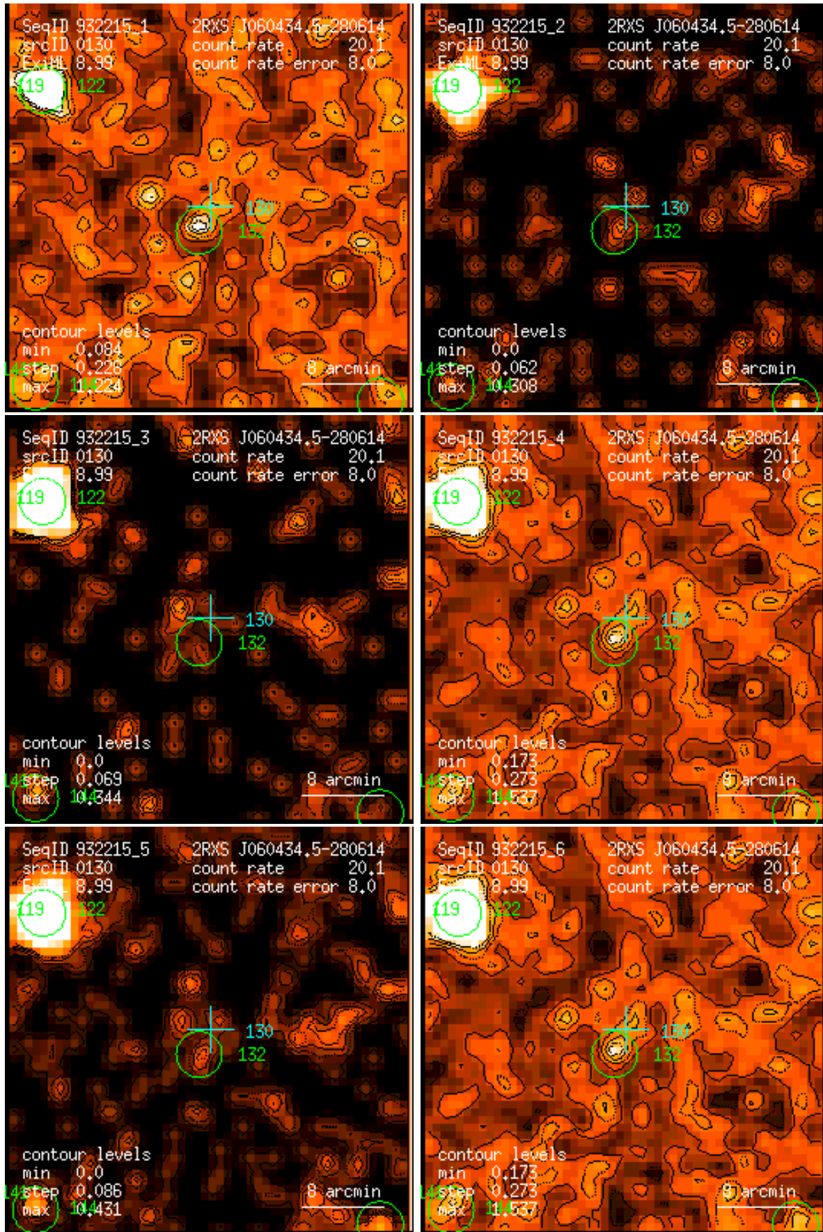
Figure 130: RASS 932215: detection 0130: band rate images, Gaussian filter: (1) PSPC channels 11 – 41, (2) 52 – 90, (3) 91 – 201, (4) 11 – 235, (5) 52 – 201, (6) 11 – 201. Broad band rates in counts/ks. Band rate contour levels in counts/ks/arcmin 2 .
