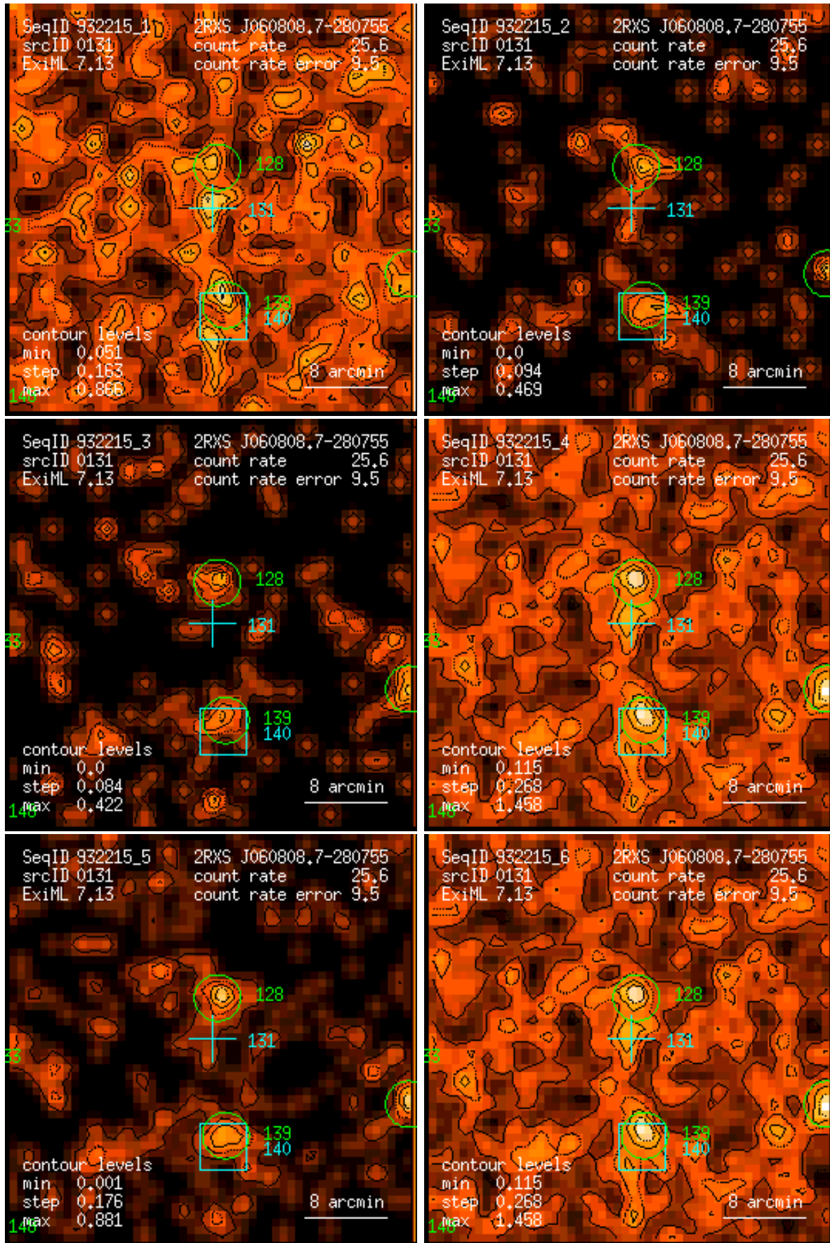
Figure 131: RASS 932215: detection 0131: band rate images, Gaussian filter: (1) PSPC channels 11 – 41, (2) 52 – 90, (3) 91 – 201, (4) 11 – 235, (5) 52 – 201, (6) 11 – 201. Broad band rates in counts/ks. Band rate contour levels in counts/ks/arcmin 2 .
