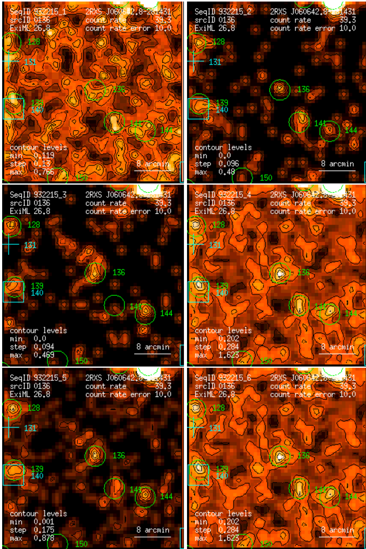
Figure 136: RASS 932215: detection 0136: band rate images, Gaussian filter: (1) PSPC channels 11 – 41, (2) 52 – 90, (3) 91 – 201, (4) 11 – 235, (5) 52 – 201, (6) 11 – 201. Broad band rates in counts/ks. Band rate contour levels in counts/ks/arcmin 2 .
