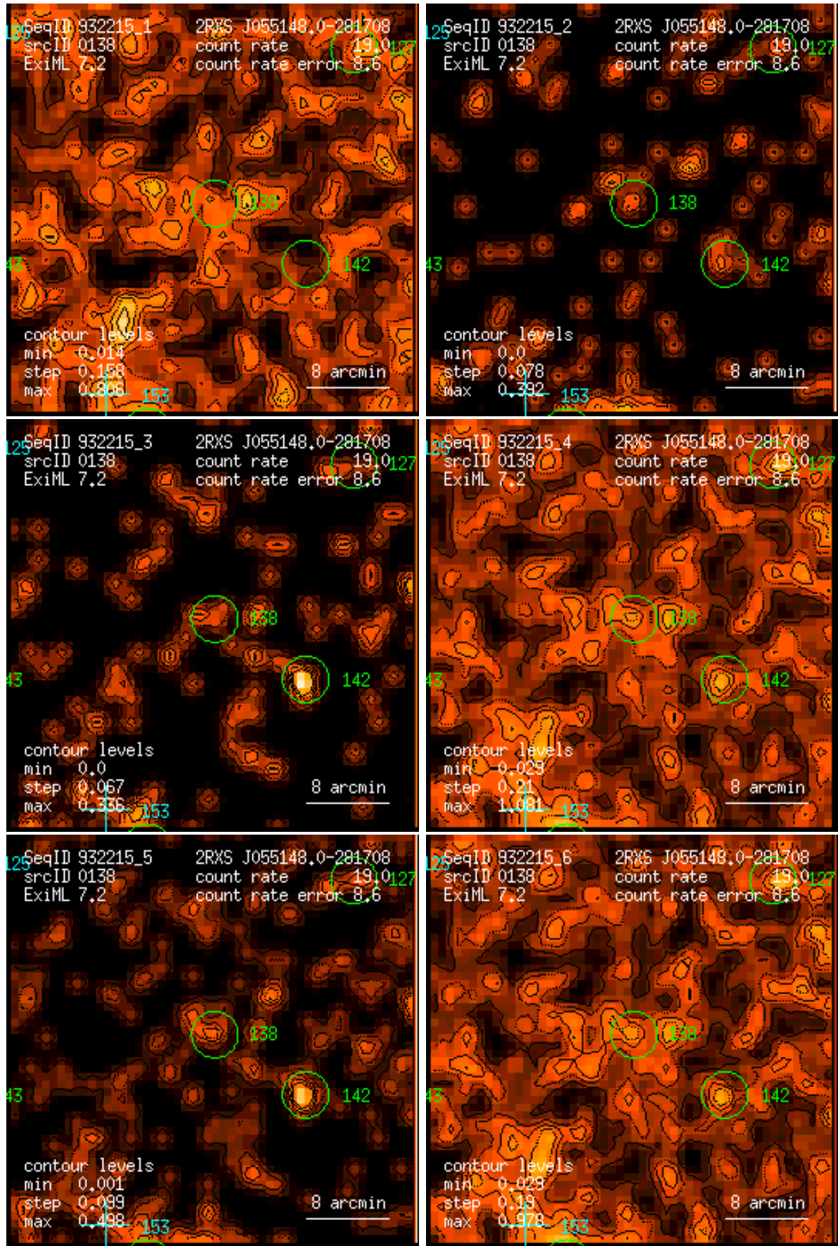
Figure 138: RASS 932215: detection 0138: band rate images, Gaussian filter: (1) PSPC channels 11 – 41, (2) 52 – 90, (3) 91 – 201, (4) 11 – 235, (5) 52 – 201, (6) 11 – 201. Broad band rates in counts/ks. Band rate contour levels in counts/ks/arcmin 2 .
