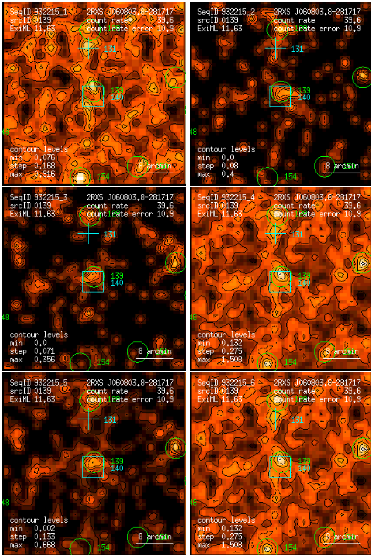
Figure 139: RASS 932215: detection 0139: band rate images, Gaussian filter: (1) PSPC channels 11 – 41, (2) 52 – 90, (3) 91 – 201, (4) 11 – 235, (5) 52 – 201, (6) 11 – 201. Broad band rates in counts/ks. Band rate contour levels in counts/ks/arcmin 2 .
