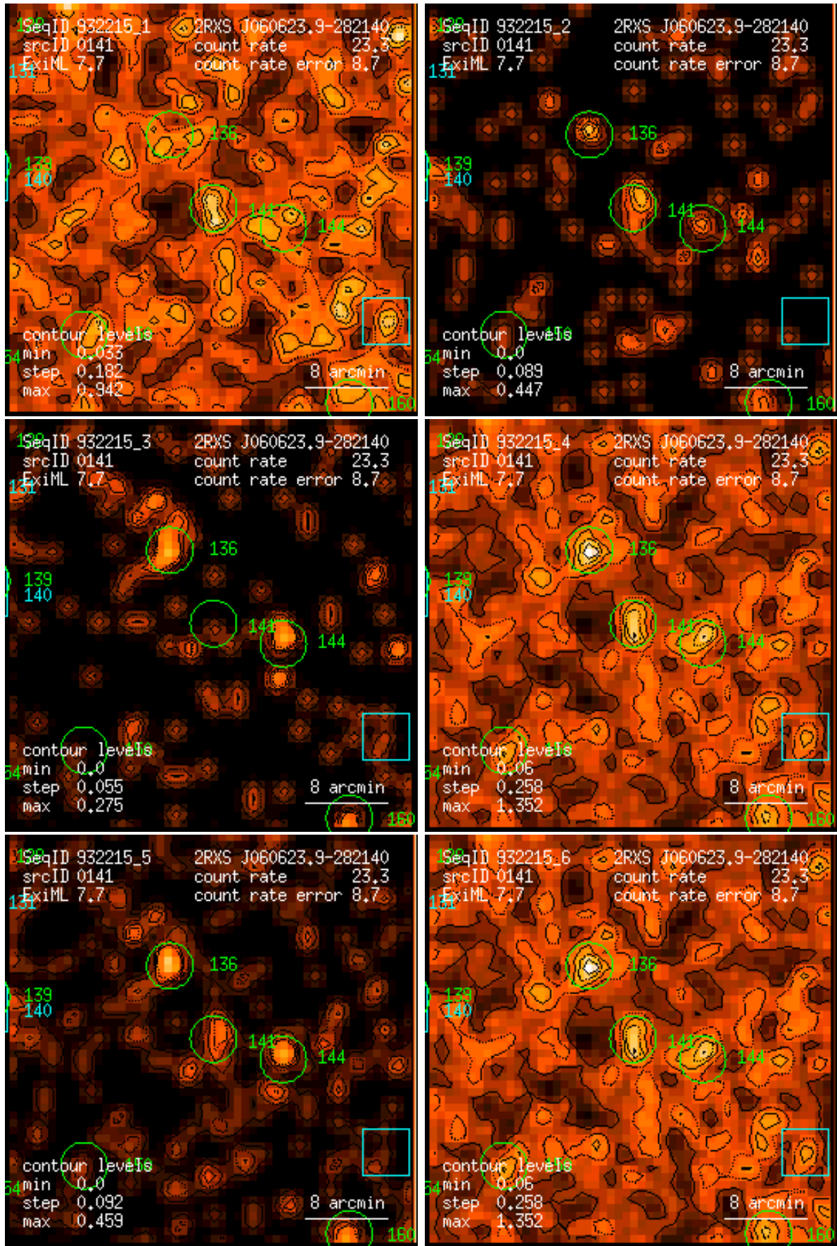
Figure 141: RASS 932215: detection 0141: band rate images, Gaussian filter: (1) PSPC channels 11 – 41, (2) 52 – 90, (3) 91 – 201, (4) 11 – 235, (5) 52 – 201, (6) 11 – 201. Broad band rates in counts/ks. Band rate contour levels in counts/ks/arcmin 2 .
