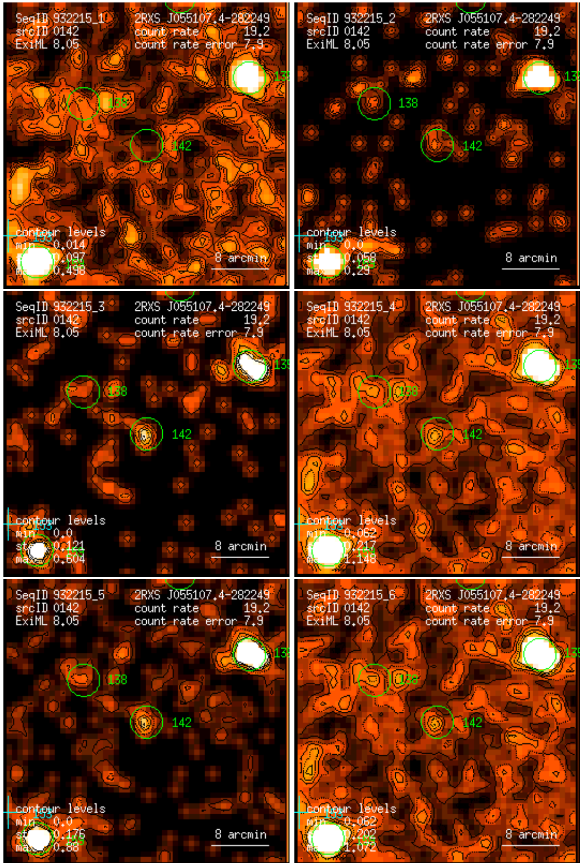
Figure 142: RASS 932215: detection 0142: band rate images, Gaussian filter: (1) PSPC channels 11 – 41, (2) 52 – 90, (3) 91 – 201, (4) 11 – 235, (5) 52 – 201, (6) 11 – 201. Broad band rates in counts/ks. Band rate contour levels in counts/ks/arcmin 2 .
