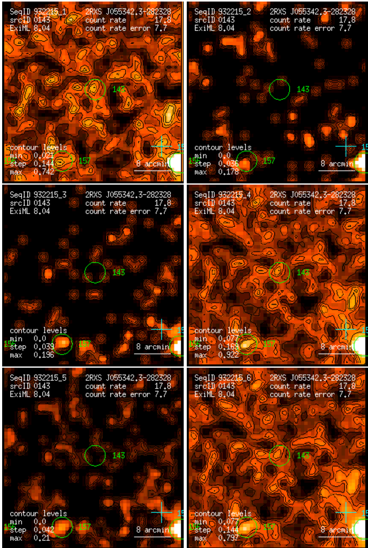
Figure 143: RASS 932215: detection 0143: band rate images, Gaussian filter: (1) PSPC channels 11 – 41, (2) 52 – 90, (3) 91 – 201, (4) 11 – 235, (5) 52 – 201, (6) 11 – 201. Broad band rates in counts/ks. Band rate contour levels in counts/ks/arcmin 2 .
