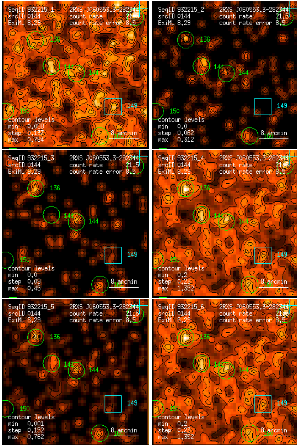
Figure 144: RASS 932215: detection 0144: band rate images, Gaussian filter: (1) PSPC channels 11 – 41, (2) 52 – 90, (3) 91 – 201, (4) 11 – 235, (5) 52 – 201, (6) 11 – 201. Broad band rates in counts/ks. Band rate contour levels in counts/ks/arcmin 2 .
