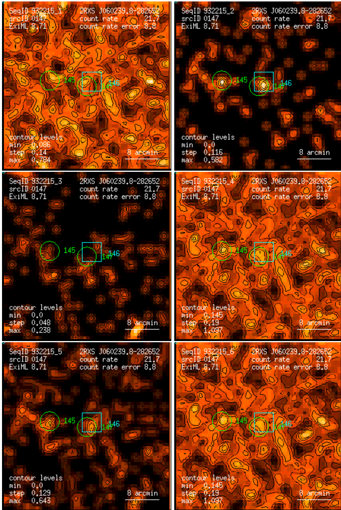
Figure 147: RASS 932215: detection 0147: band rate images, Gaussian filter: (1) PSPC channels 11 – 41, (2) 52 – 90, (3) 91 – 201, (4) 11 – 235, (5) 52 – 201, (6) 11 – 201. Broad band rates in counts/ks. Band rate contour levels in counts/ks/arcmin 2 .
