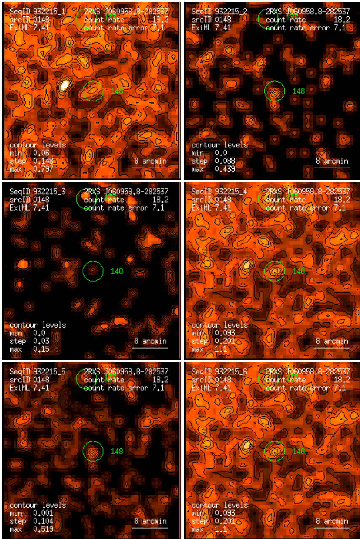
Figure 148: RASS 932215: detection 0148: band rate images, Gaussian filter: (1) PSPC channels 11 – 41, (2) 52 – 90, (3) 91 – 201, (4) 11 – 235, (5) 52 – 201, (6) 11 – 201. Broad band rates in counts/ks. Band rate contour levels in counts/ks/arcmin 2 .
