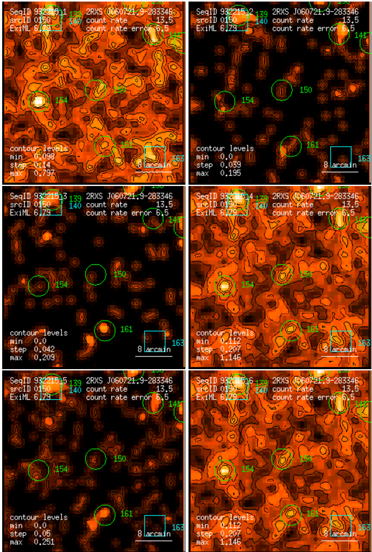
Figure 150: RASS 932215: detection 0150: band rate images, Gaussian filter: (1) PSPC channels 11 – 41, (2) 52 – 90, (3) 91 – 201, (4) 11 – 235, (5) 52 – 201, (6) 11 – 201. Broad band rates in counts/ks. Band rate contour levels in counts/ks/arcmin 2 .
