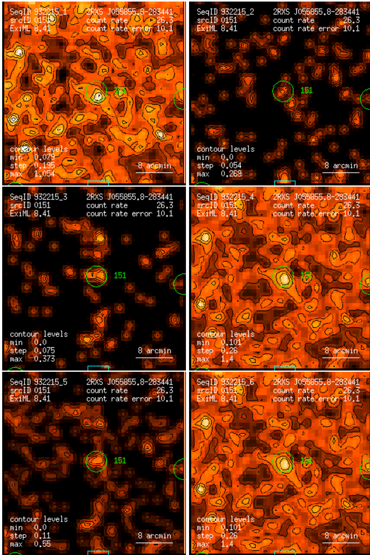
Figure 151: RASS 932215: detection 0151: band rate images, Gaussian filter: (1) PSPC channels 11 – 41, (2) 52 – 90, (3) 91 – 201, (4) 11 – 235, (5) 52 – 201, (6) 11 – 201. Broad band rates in counts/ks. Band rate contour levels in counts/ks/arcmin 2 .
