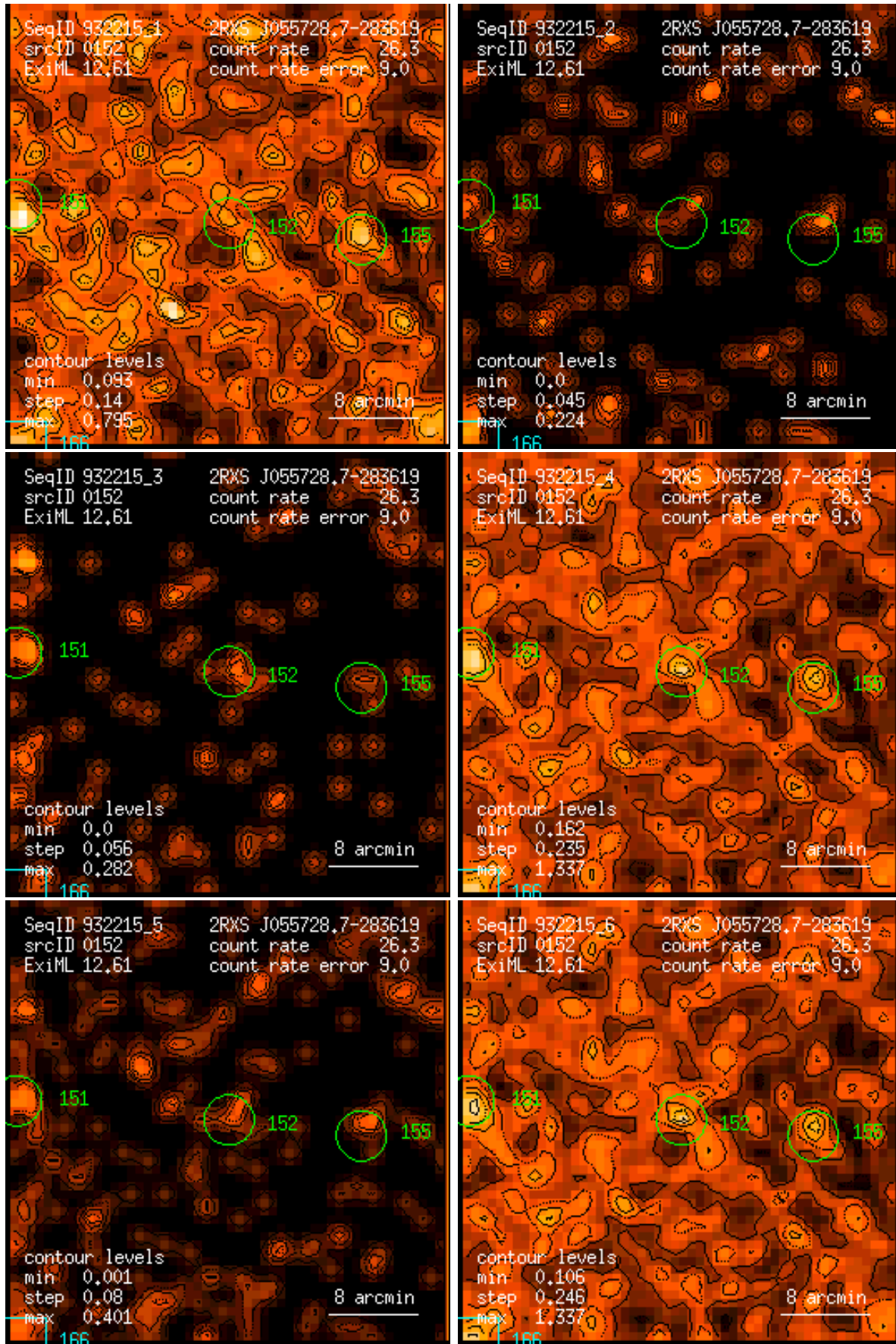
Figure 152: RASS 932215: detection 0152: band rate images, Gaussian filter: (1) PSPC channels 11 – 41, (2) 52 – 90, (3) 91 – 201, (4) 11 – 235, (5) 52 – 201, (6) 11 – 201. Broad band rates in counts/ks. Band rate contour levels in counts/ks/arcmin 2 .
