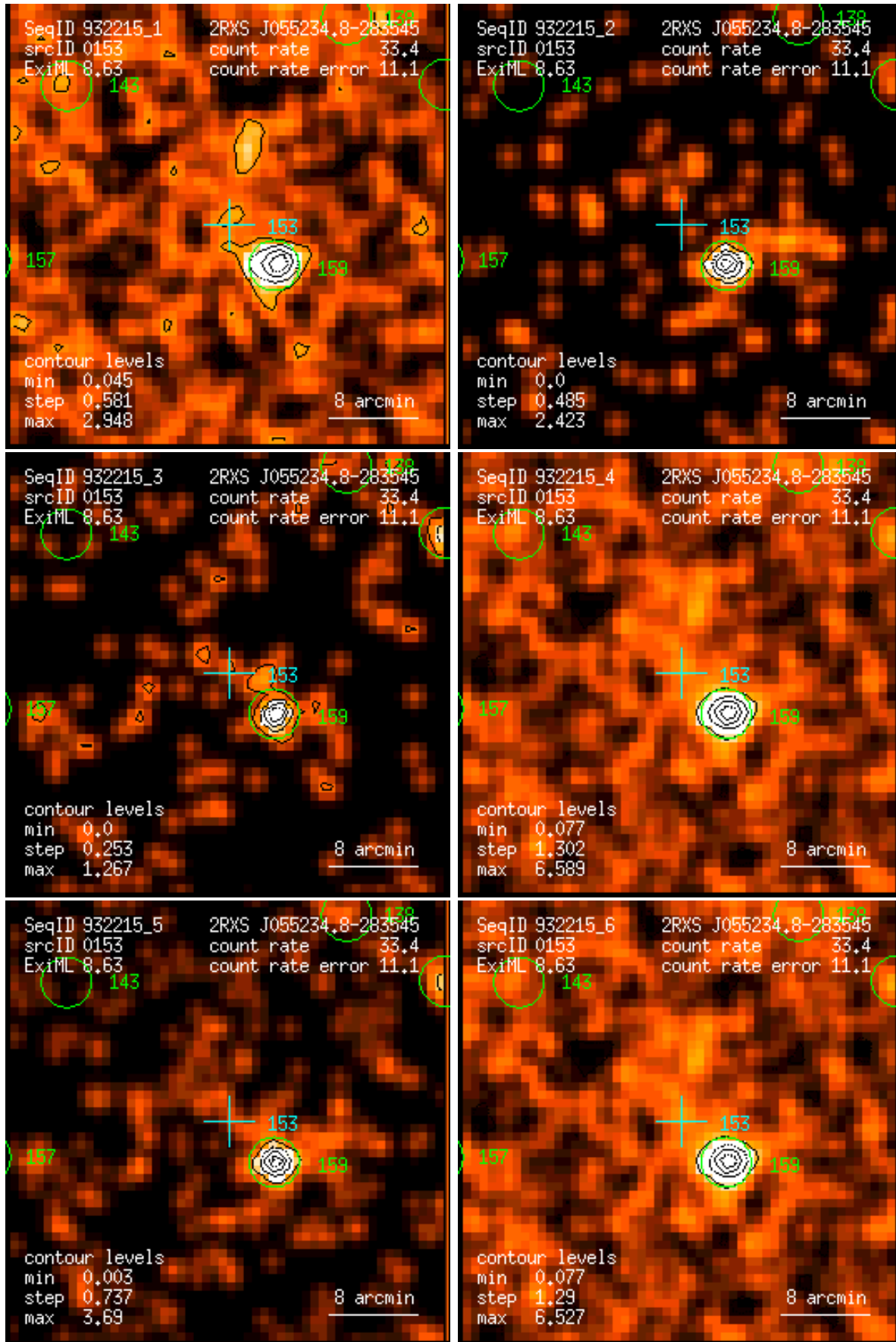
Figure 153: RASS 932215: detection 0153: band rate images, Gaussian filter: (1) PSPC channels 11 – 41, (2) 52 – 90, (3) 91 – 201, (4) 11 – 235, (5) 52 – 201, (6) 11 – 201. Broad band rates in counts/ks. Band rate contour levels in counts/ks/arcmin 2 .
