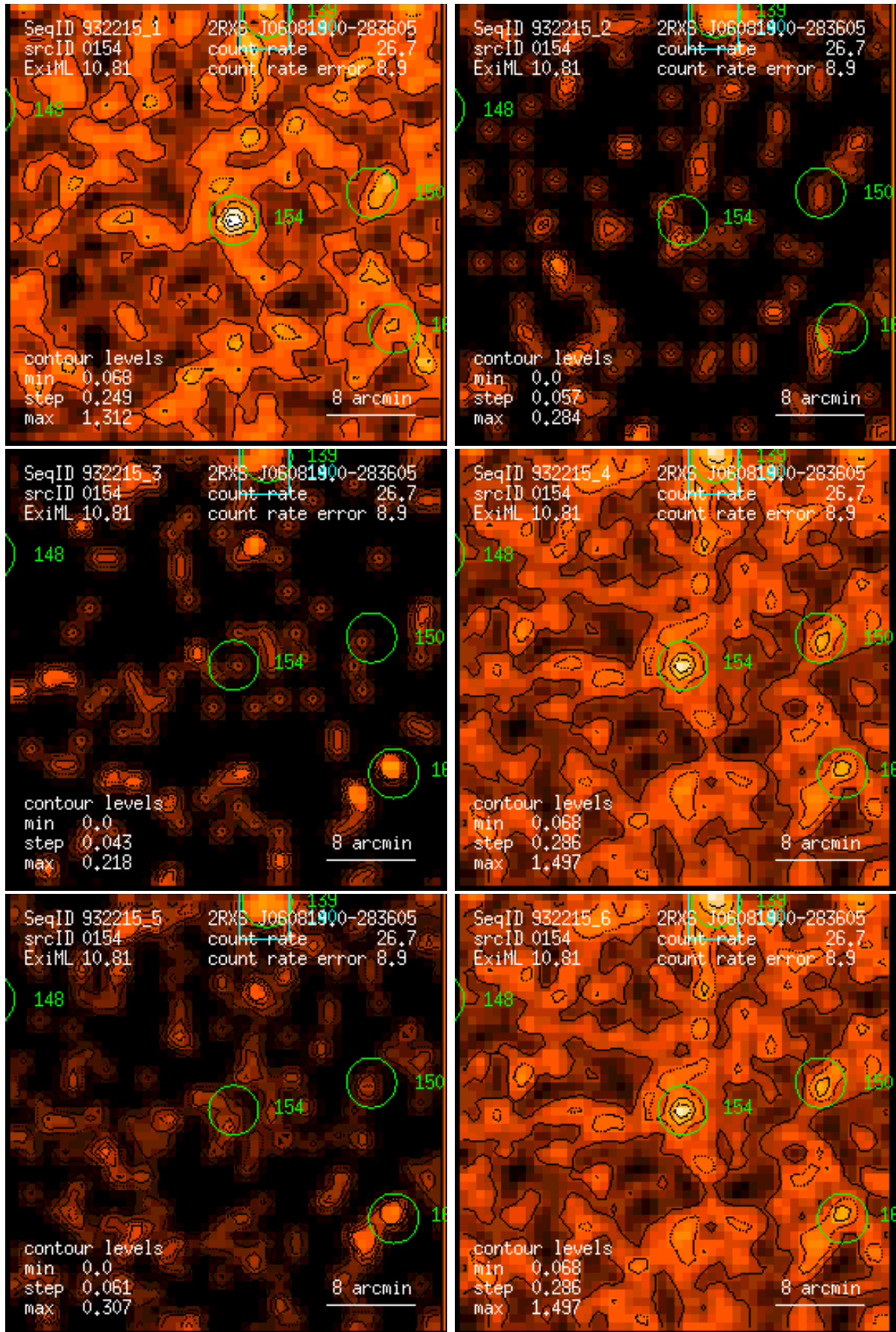
Figure 154: RASS 932215: detection 0154: band rate images, Gaussian filter: (1) PSPC channels 11 – 41, (2) 52 – 90, (3) 91 – 201, (4) 11 – 235, (5) 52 – 201, (6) 11 – 201. Broad band rates in counts/ks. Band rate contour levels in counts/ks/arcmin 2 .
