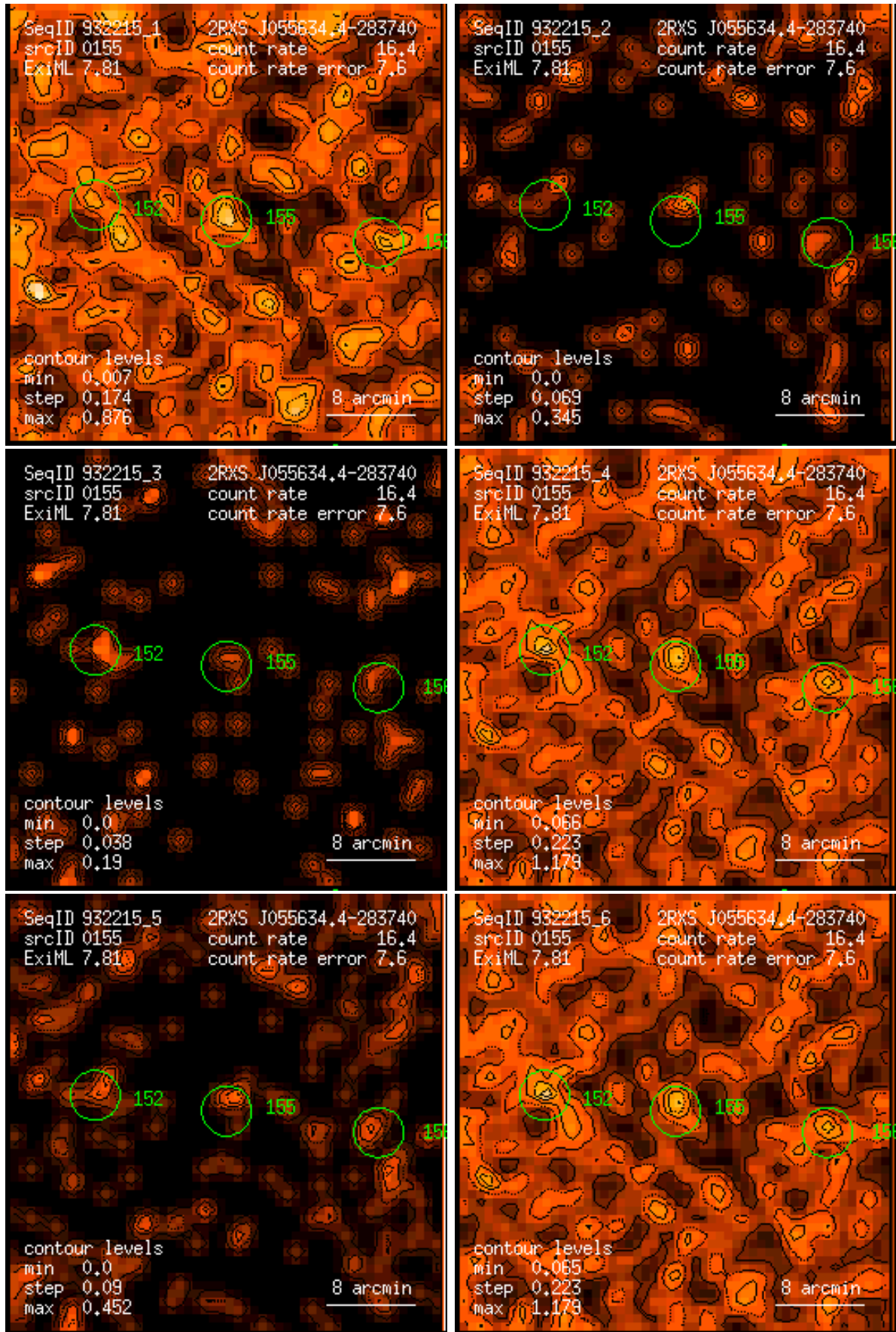
Figure 155: RASS 932215: detection 0155: band rate images, Gaussian filter: (1) PSPC channels 11 – 41, (2) 52 – 90, (3) 91 – 201, (4) 11 – 235, (5) 52 – 201, (6) 11 – 201. Broad band rates in counts/ks. Band rate contour levels in counts/ks/arcmin 2 .
