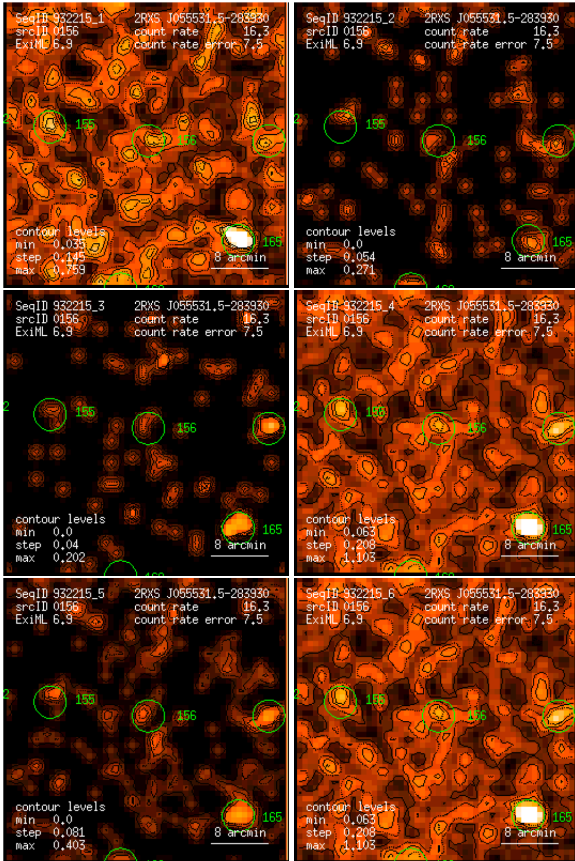
Figure 156: RASS 932215: detection 0156: band rate images, Gaussian filter: (1) PSPC channels 11 – 41, (2) 52 – 90, (3) 91 – 201, (4) 11 – 235, (5) 52 – 201, (6) 11 – 201. Broad band rates in counts/ks. Band rate contour levels in counts/ks/arcmin 2 .
