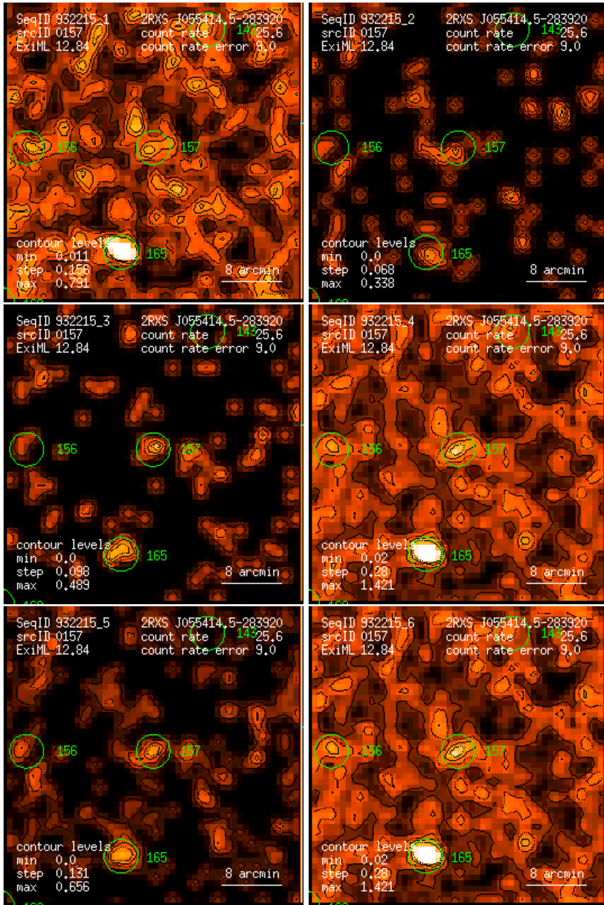
Figure 157: RASS 932215: detection 0157: band rate images, Gaussian filter: (1) PSPC channels 11 – 41, (2) 52 – 90, (3) 91 – 201, (4) 11 – 235, (5) 52 – 201, (6) 11 – 201. Broad band rates in counts/ks. Band rate contour levels in counts/ks/arcmin 2 .
